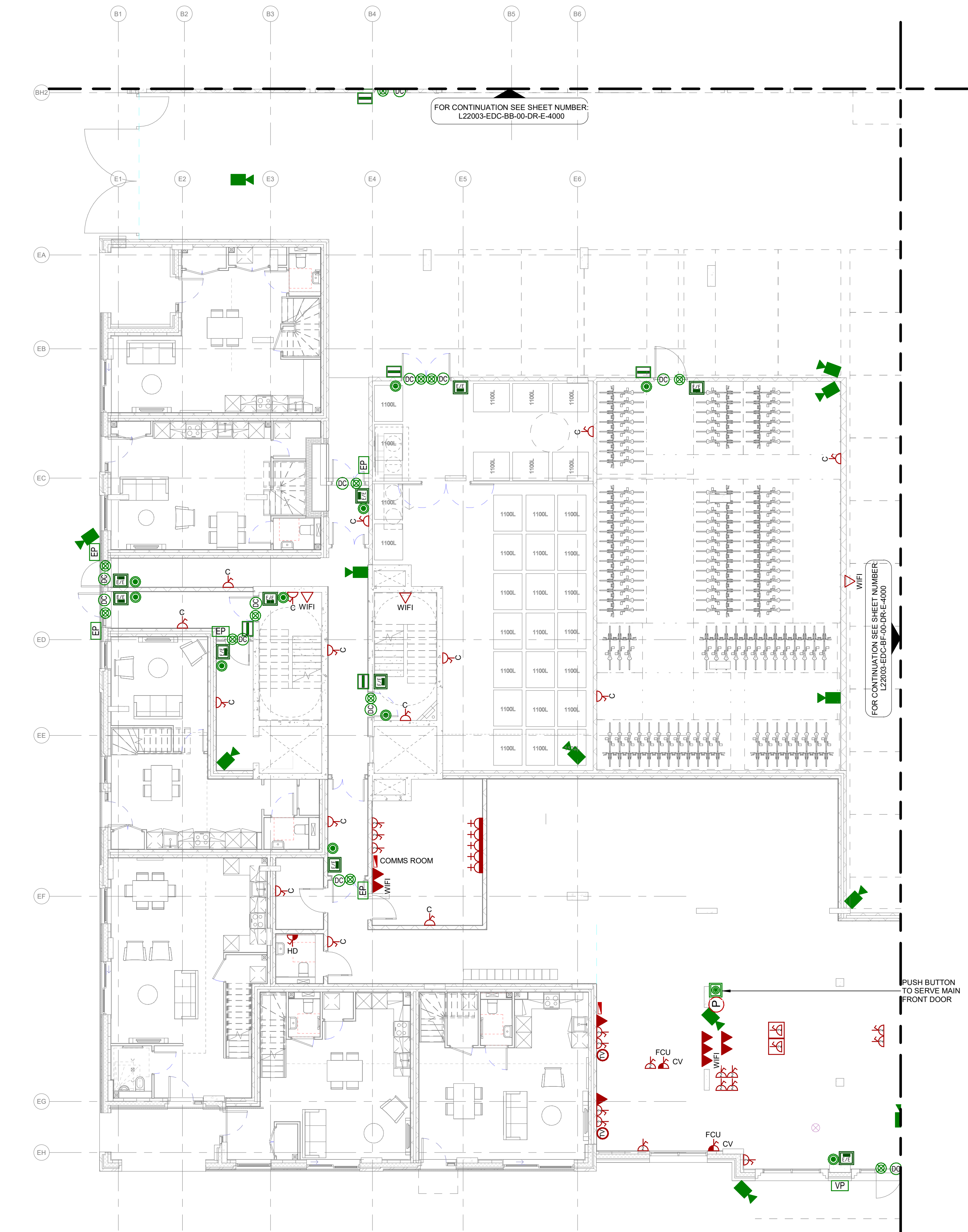
1 Block E - Ground Floor - General Services Layout 1 : 100
