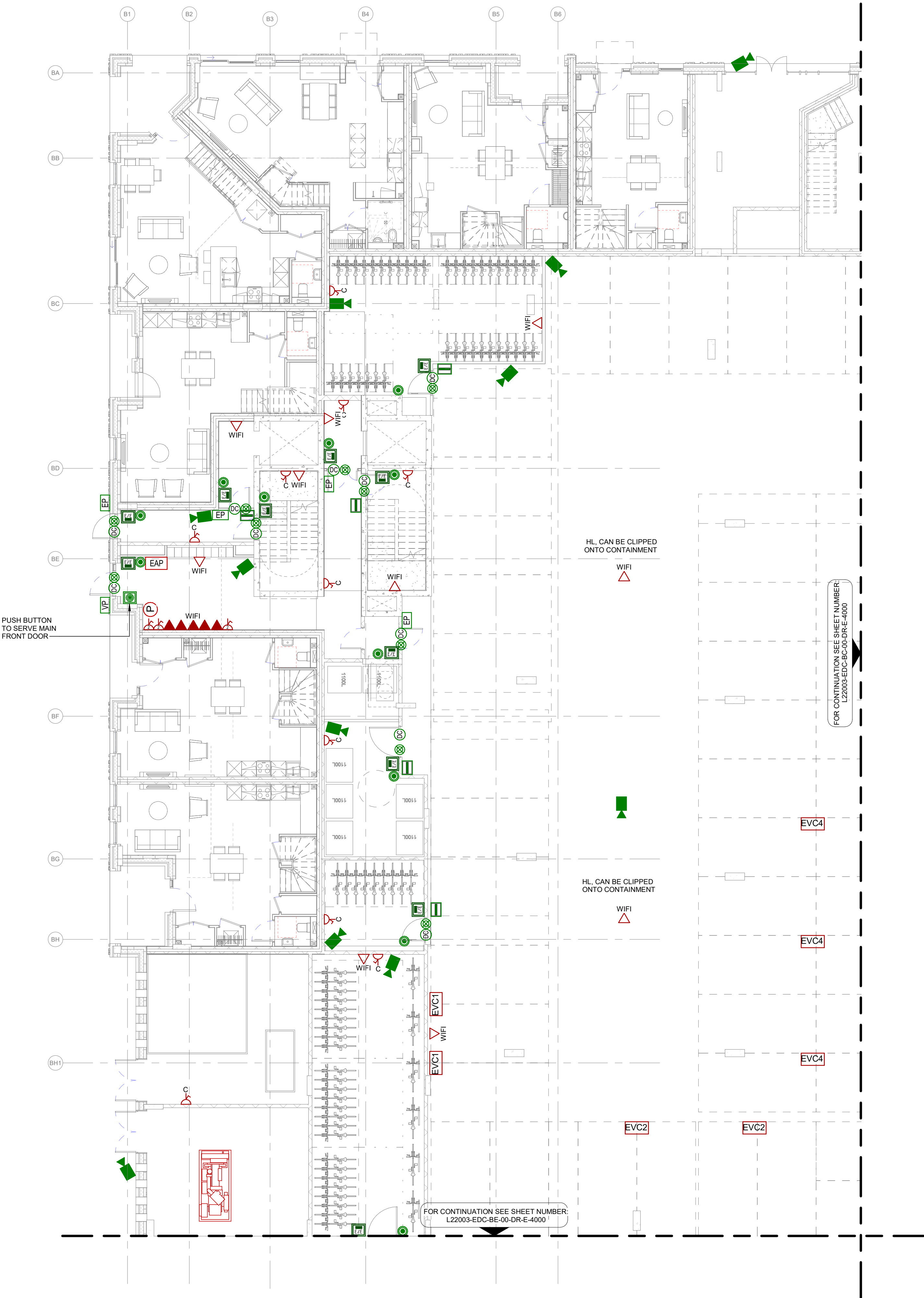
1 Block B - Ground Floor - General Services Layout 1 : 100
