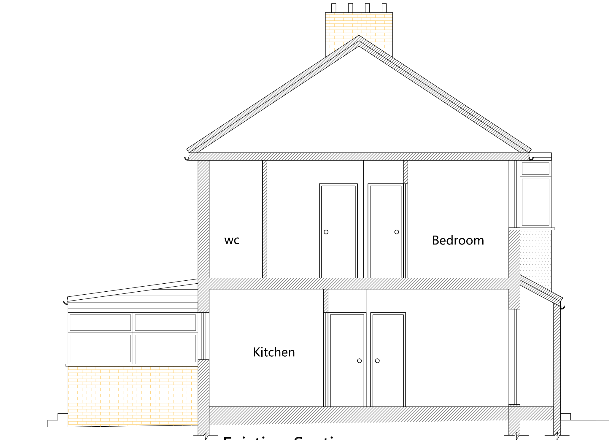
Existing Section x-x
