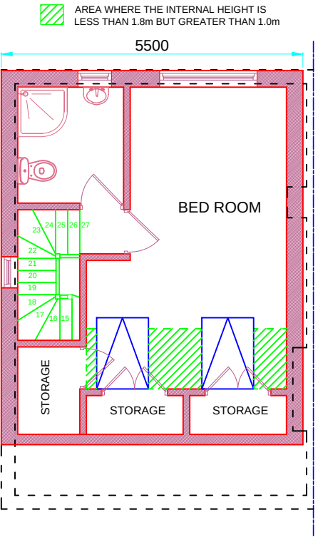
PROPOSED LOFT FLOOR PLAN Scale 1:100
