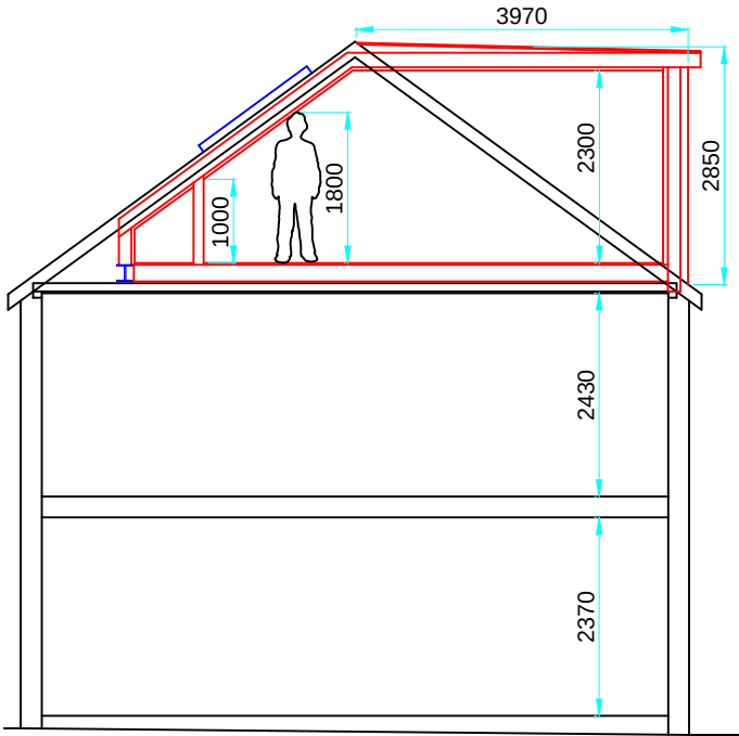
PROPOSED SECTION Scale 1:100
