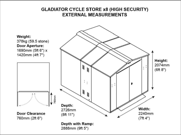
Example - Asgard Gladiator Cycle store - 8 bikes
