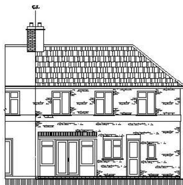
Existing West Elevation Scale 1:100
