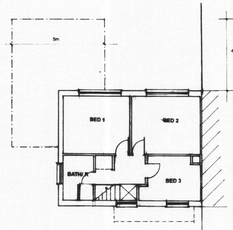
FIRST FLOOR PROPOSED
