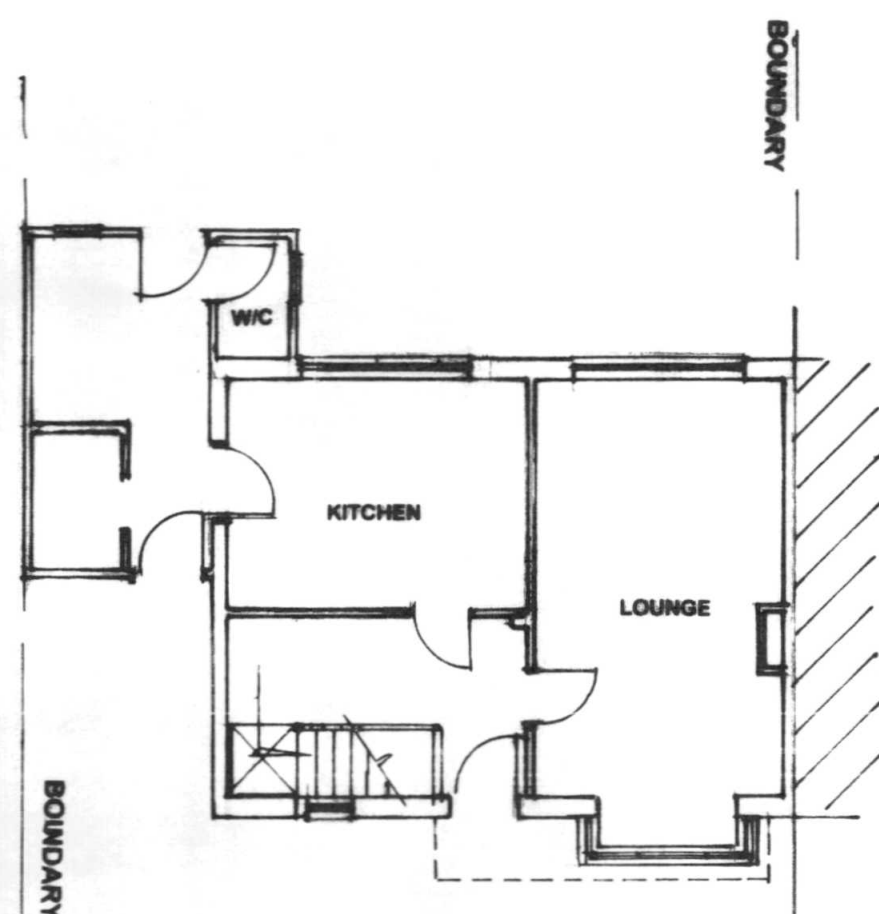
PLAN EXISTING SCALE 1-100
