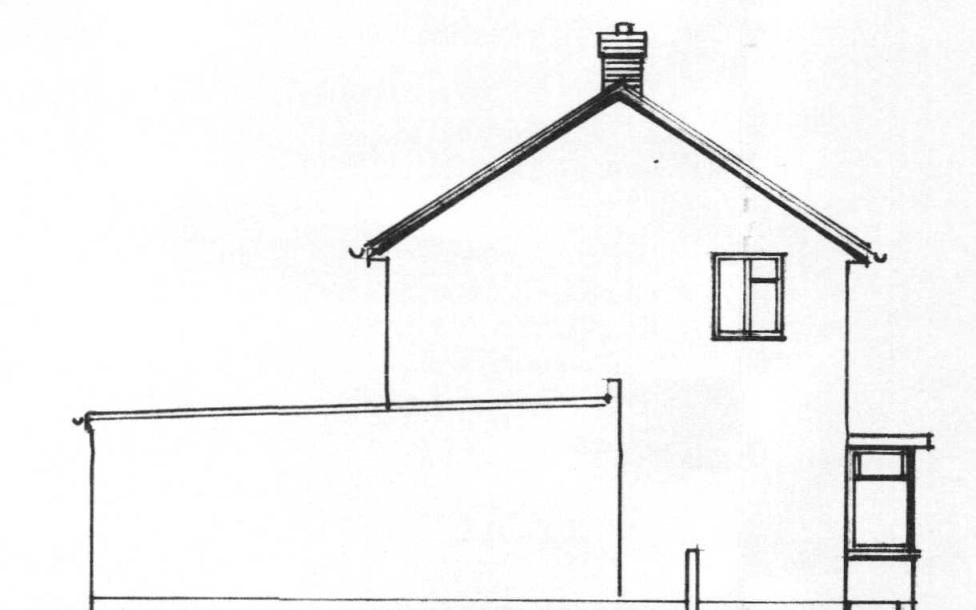
LEFT FLANK PROPOSED
