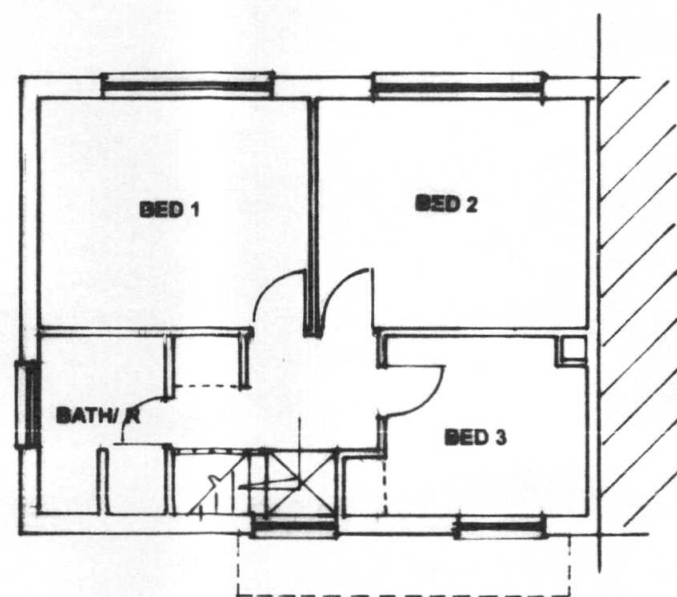
FIRST FLOOR EXISTING
