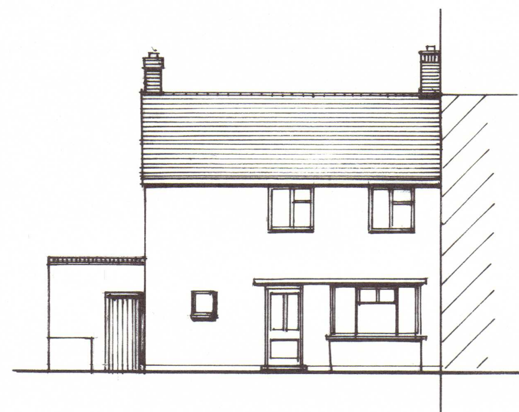
FRONT ELEV EXISTING
