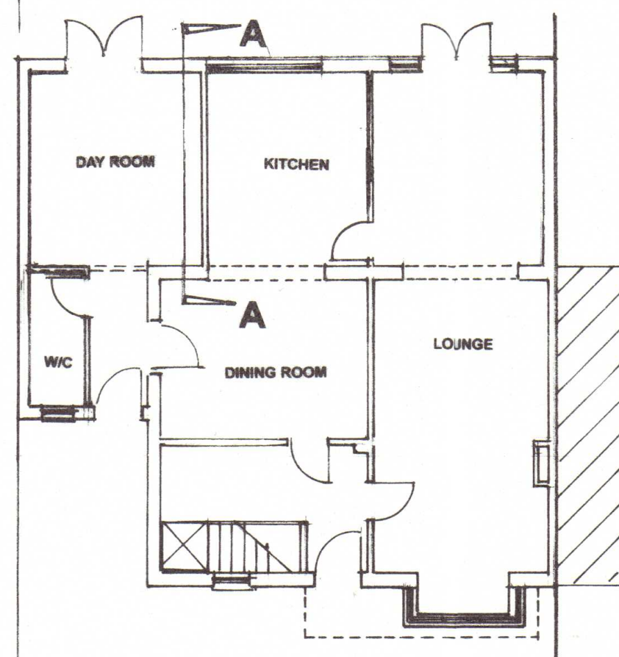
PLAN PROPOSED
