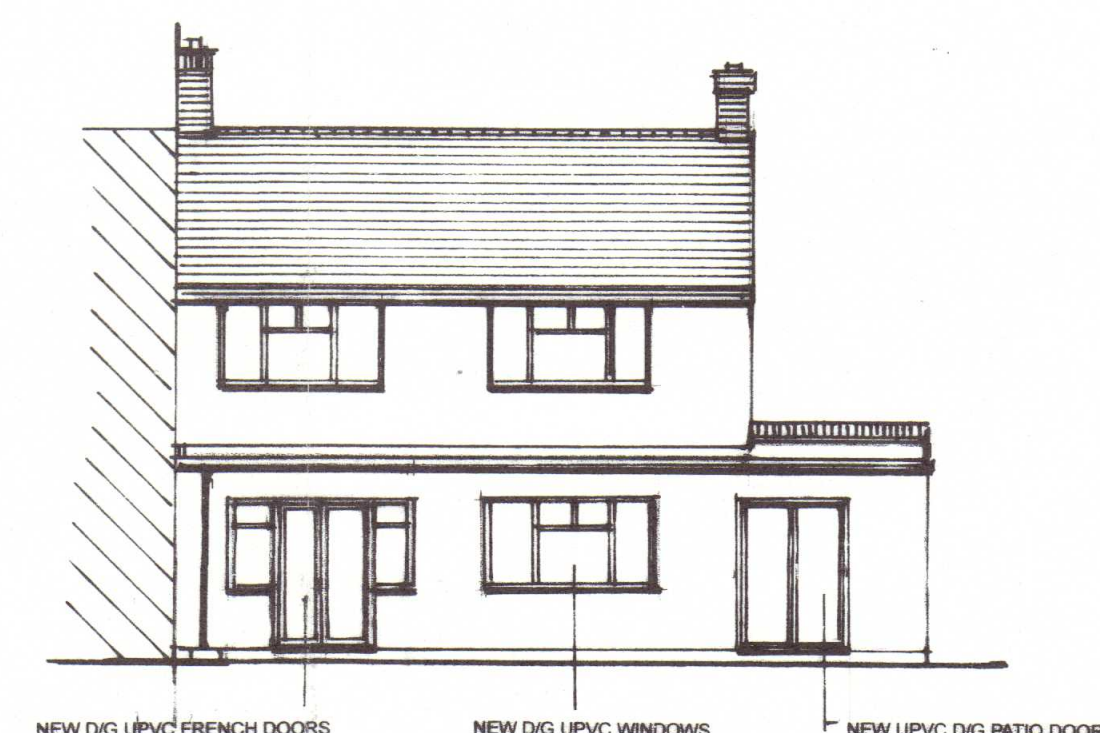
REAR ELEV PROPOSED
