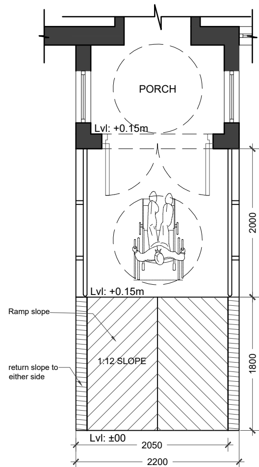
01 - PART RAMP PLAN
