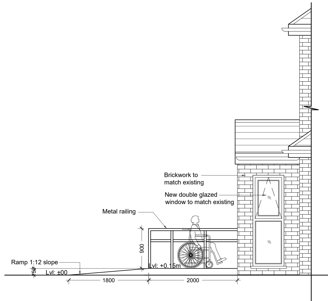
02 -PART SIDE ELEVATION
