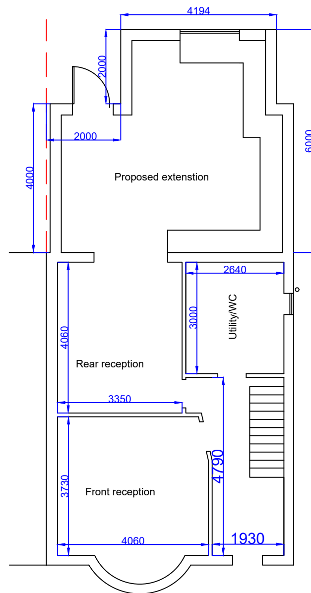
Ground floor plans
