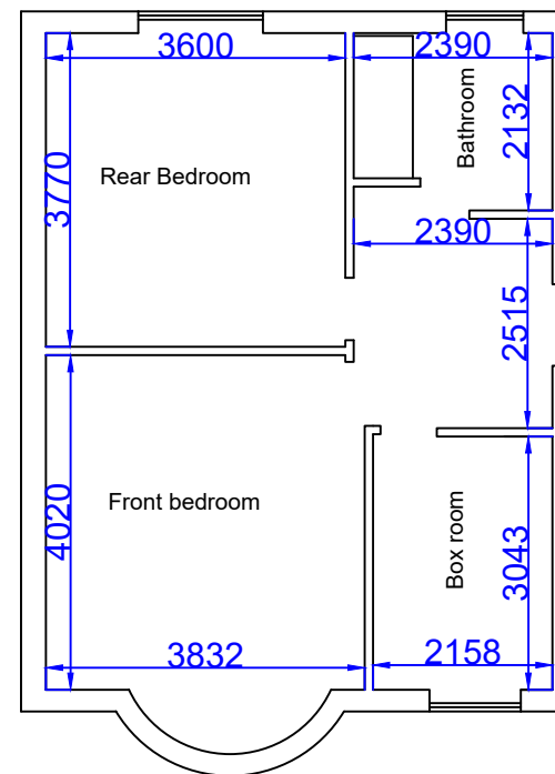
First floor plans
