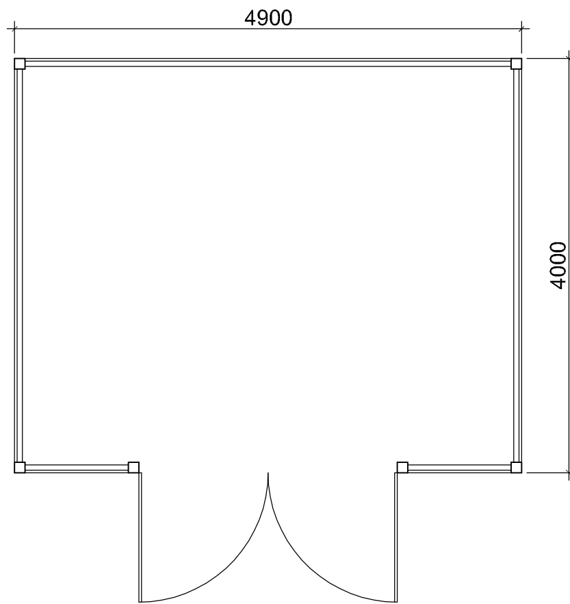
PLAN
