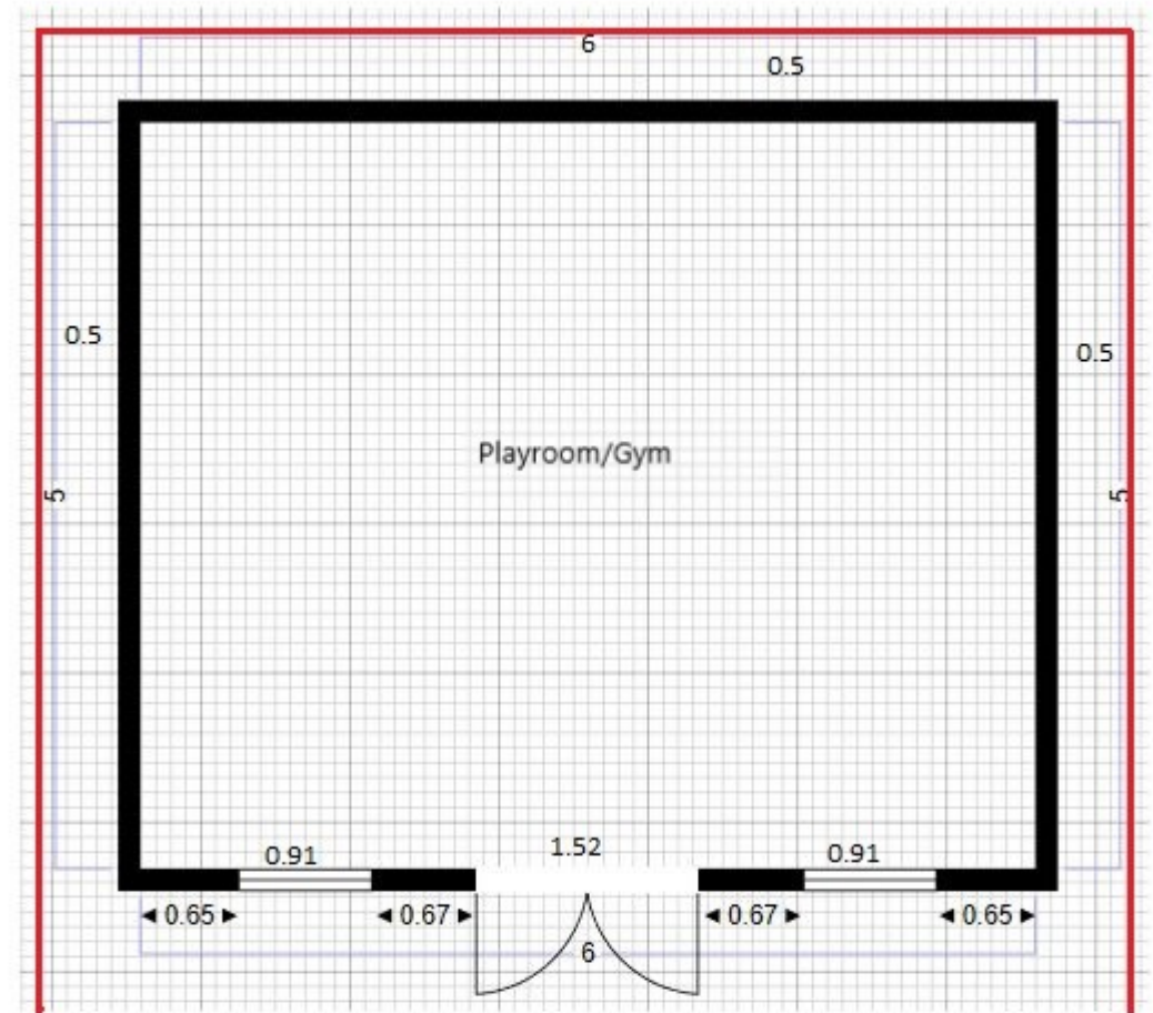
FLOORPLAN SCALE 1/50
