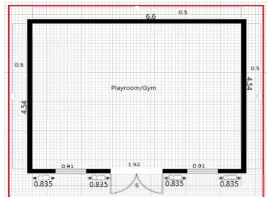
FLOORPLAN SCALE 1/50
