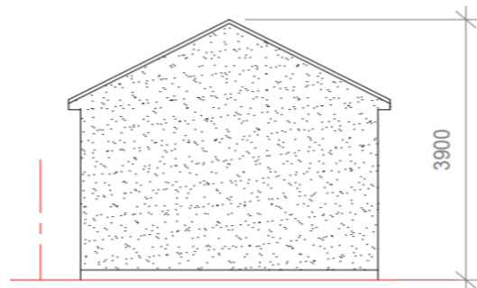
Proposed Outbuilding Side Elevation Scale 1:100
