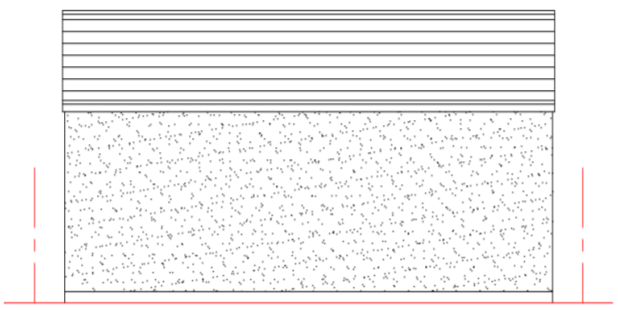
Proposed Outbuilding Rear Elevation Scale 1:100
