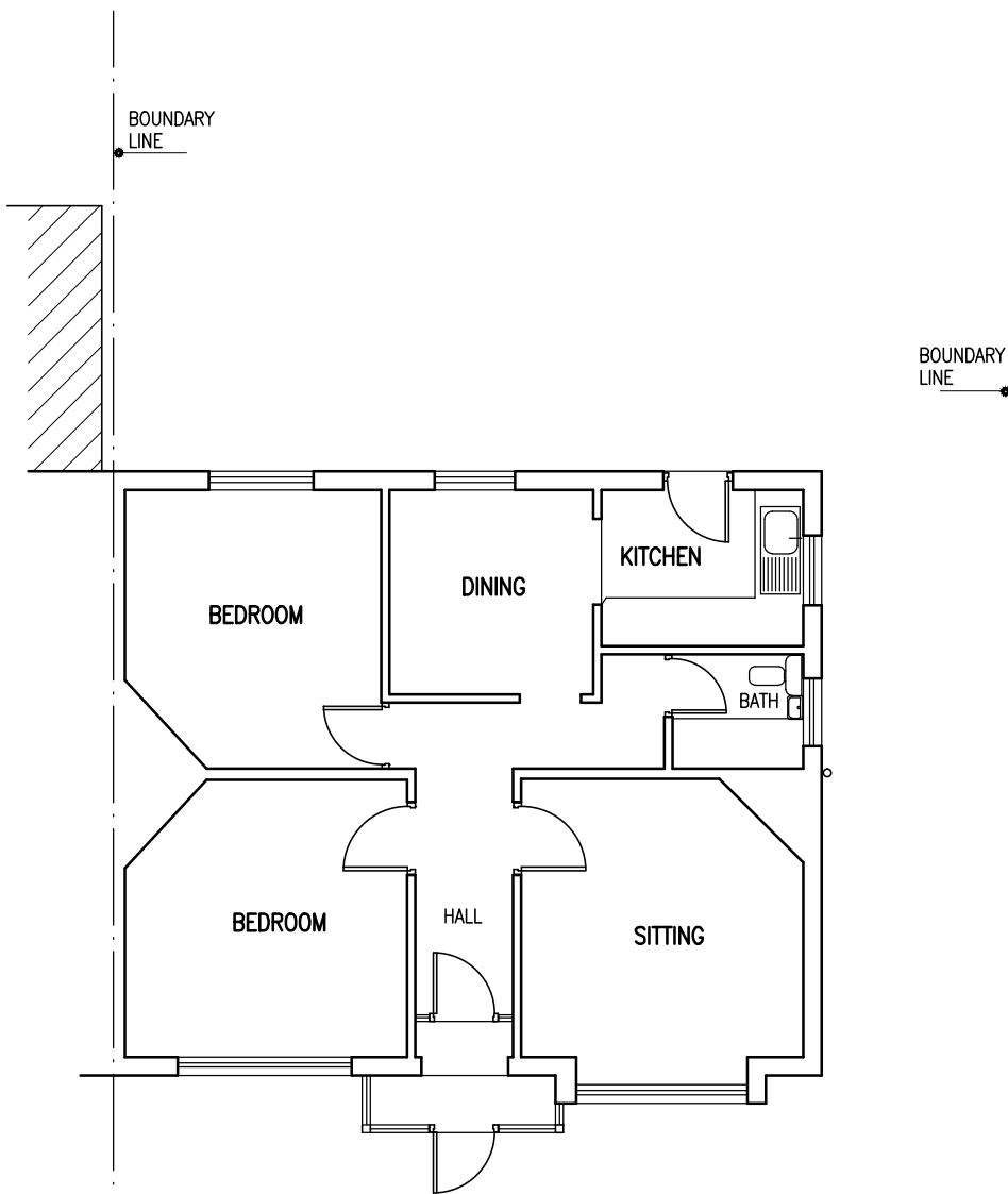
FLOOR PLAN EXISTING
