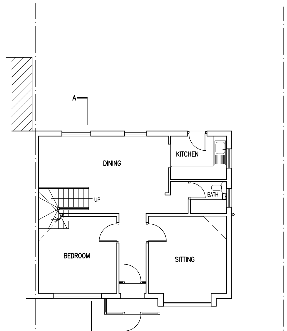
FLOOR PLAN PROPOSED
