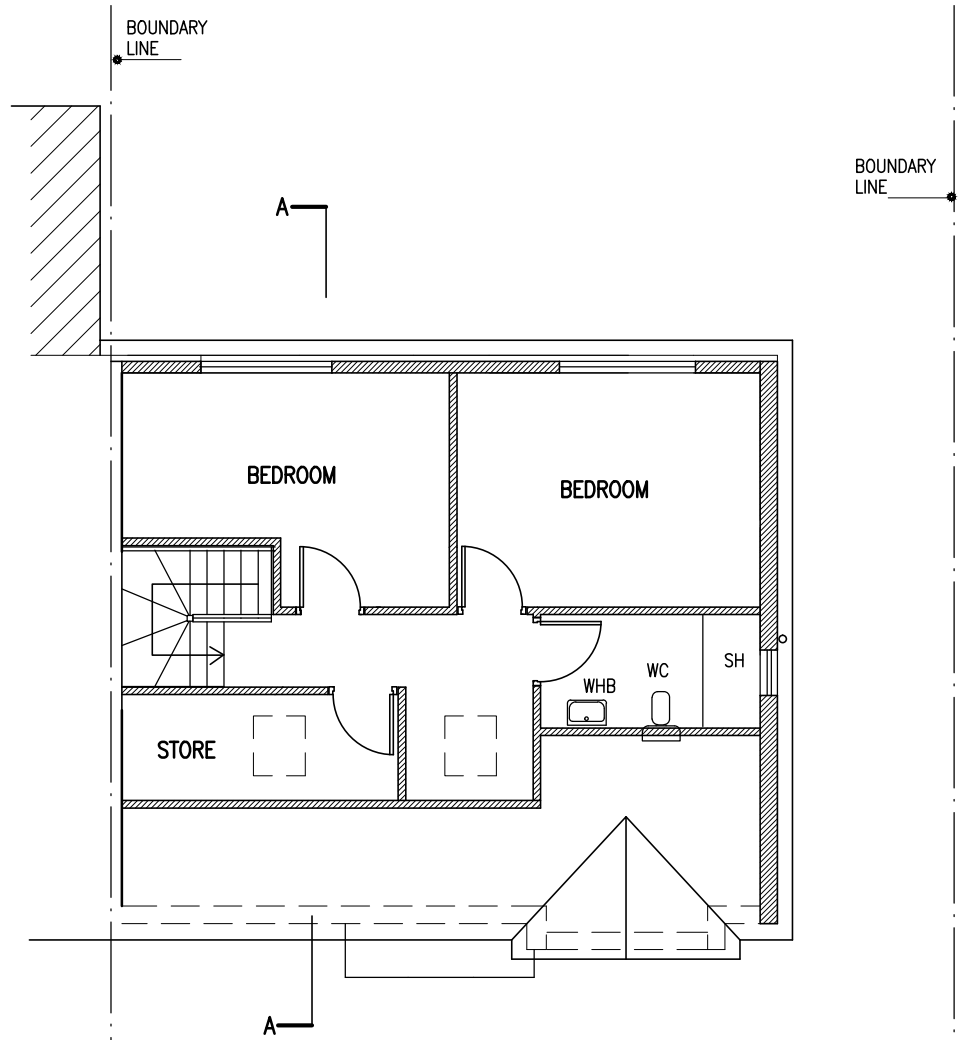
LOFT FLOOR PLAN PROPOSED
