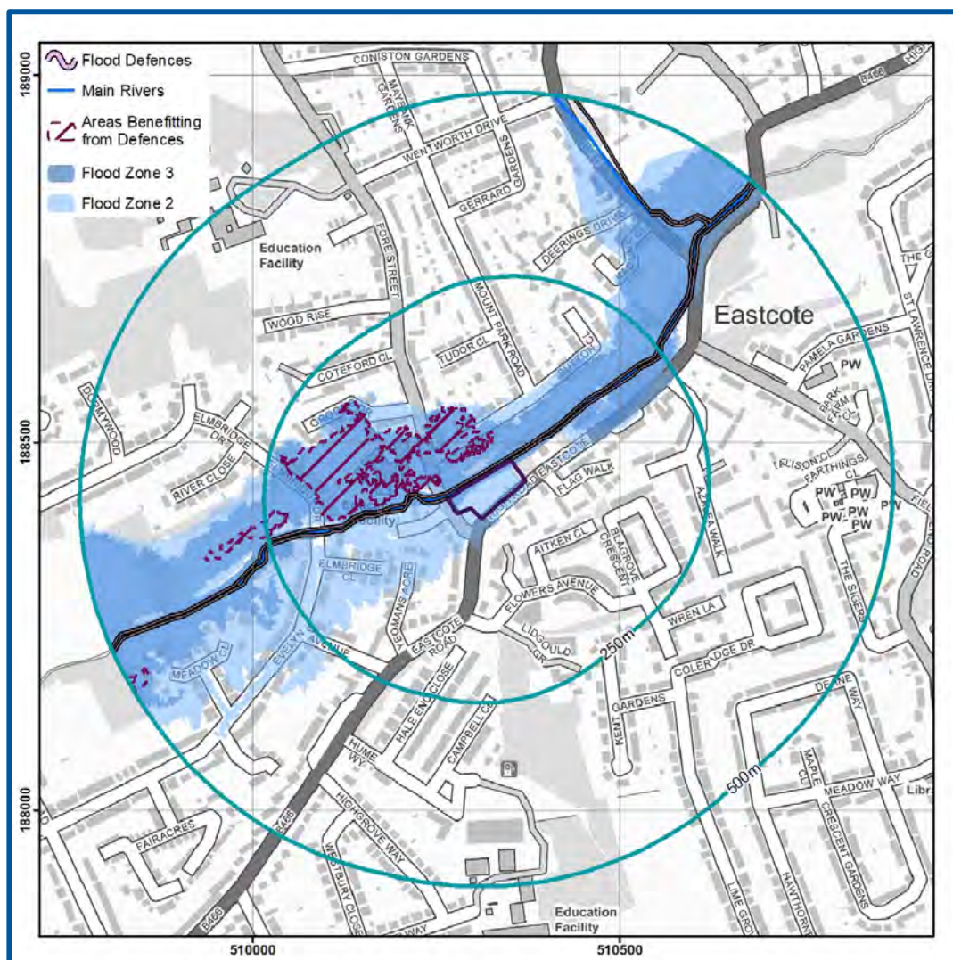
Figure 6. EA Flood Map for Planning Purposes (EA, 2023)
