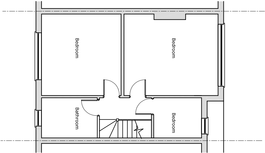
Existing First Floor Layout
