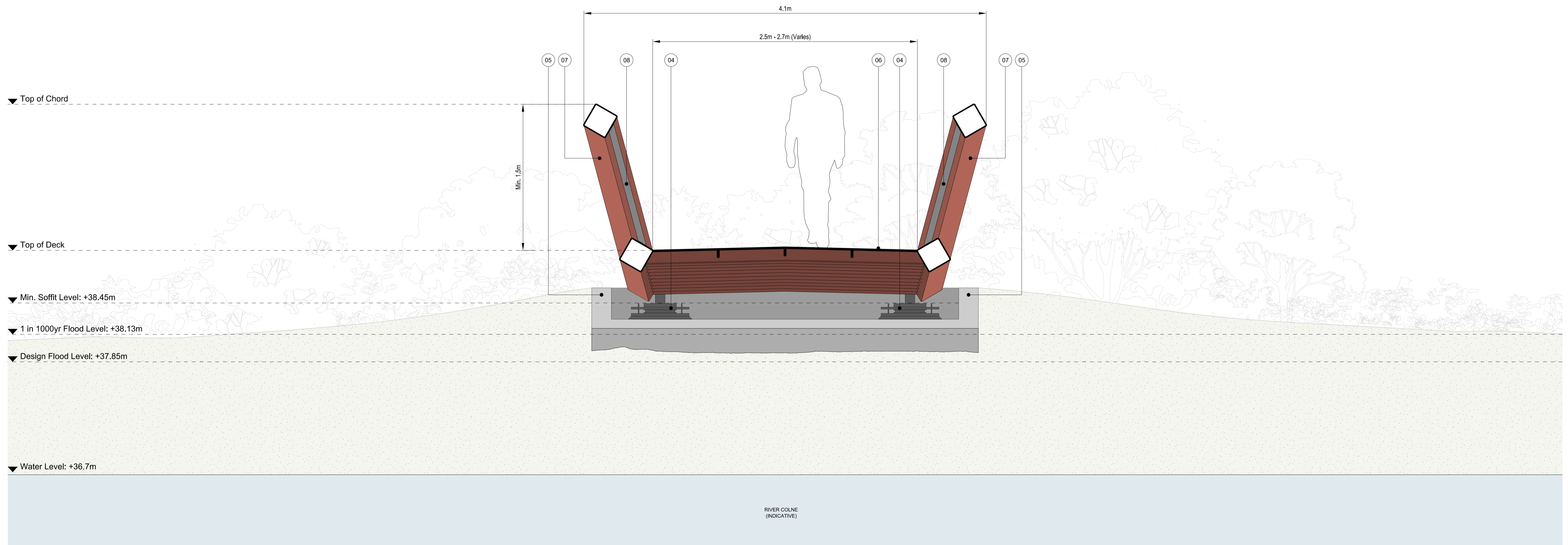
B Proposed Section 128105 Scale 1:20 @ A1
