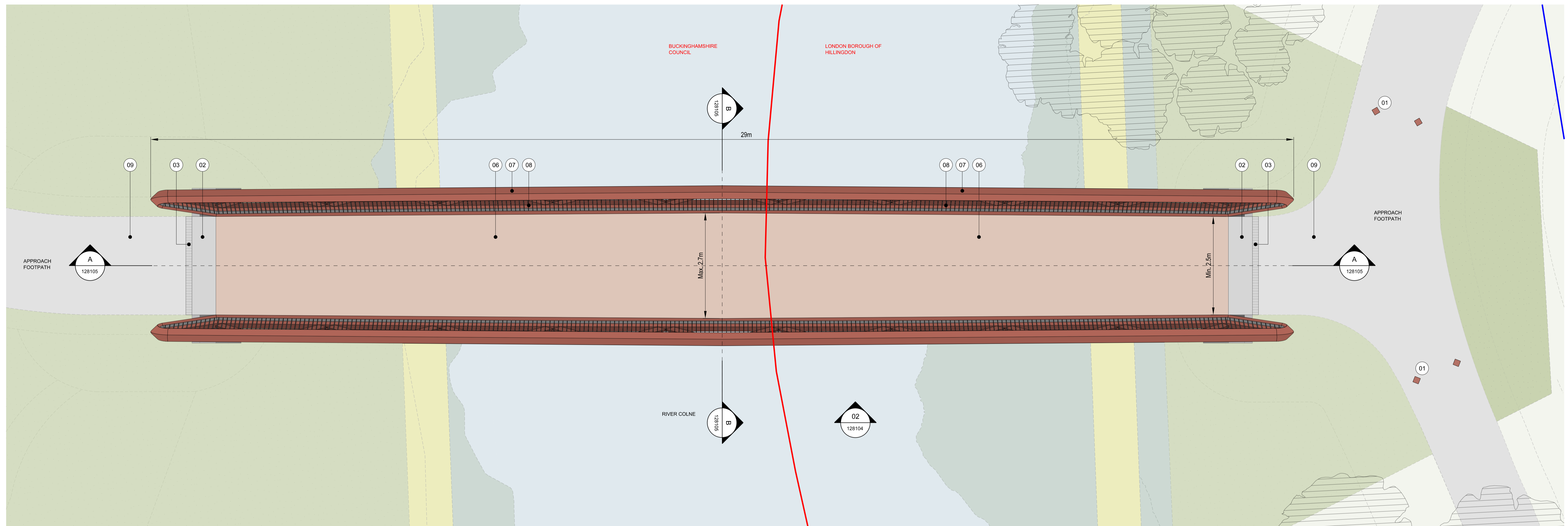
01 General Arrangement Plan 128104 Scale 1:50 @ A1
