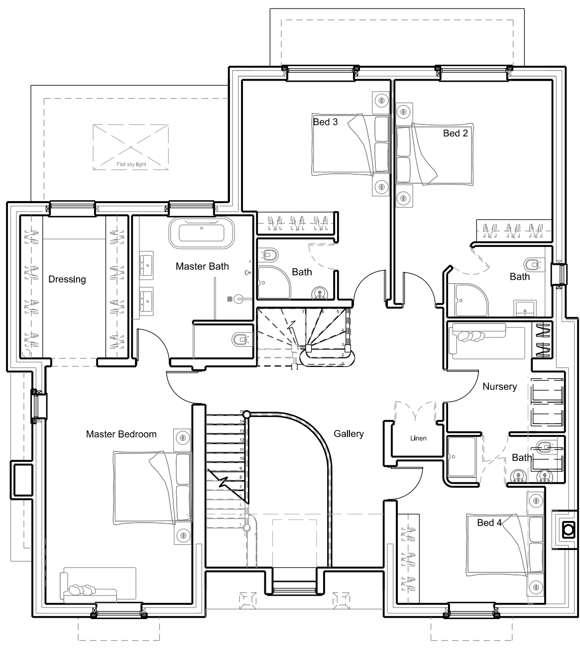
First Floor
