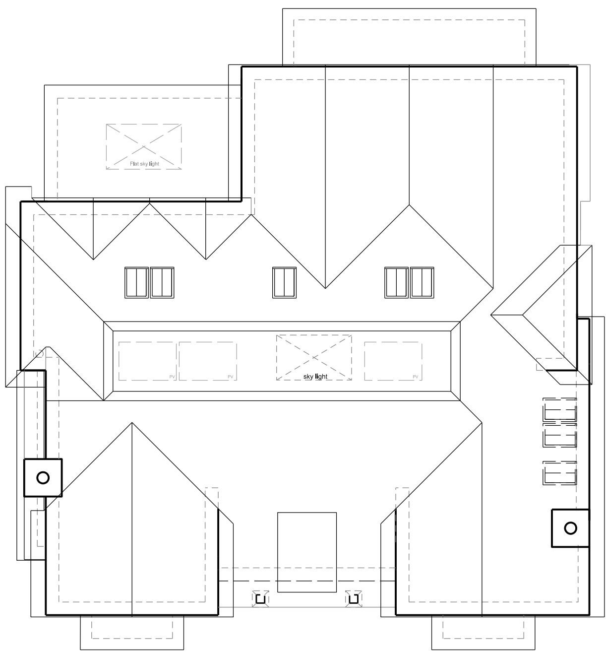
Roof Plan
