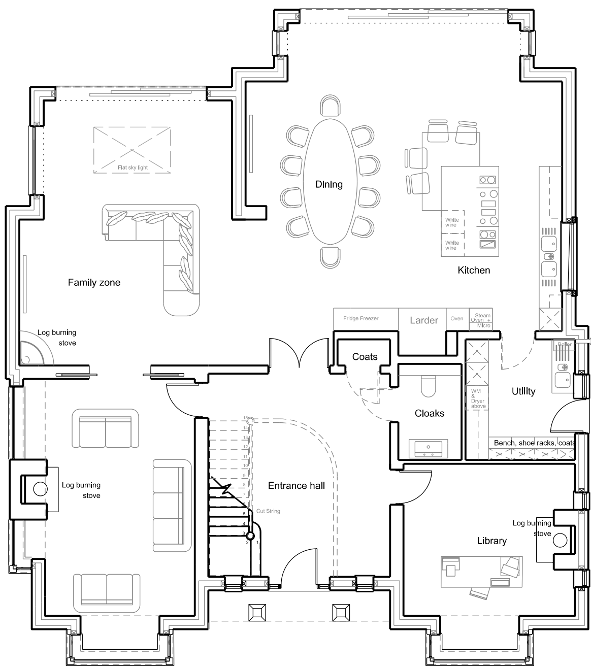
Ground Floor
