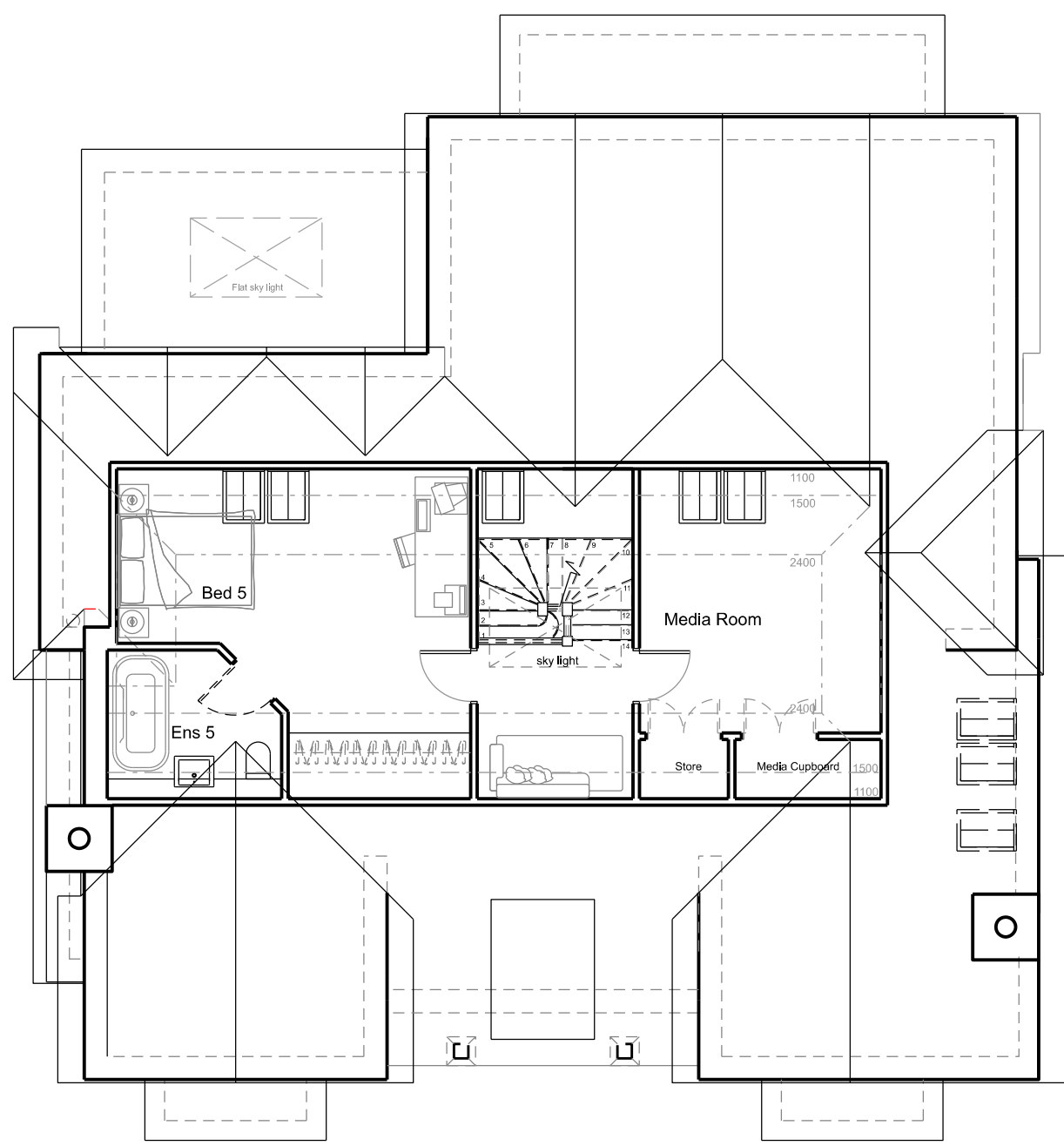
Attic Plan
