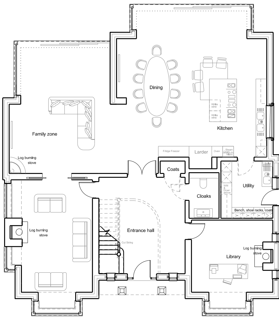
Ground Floor
