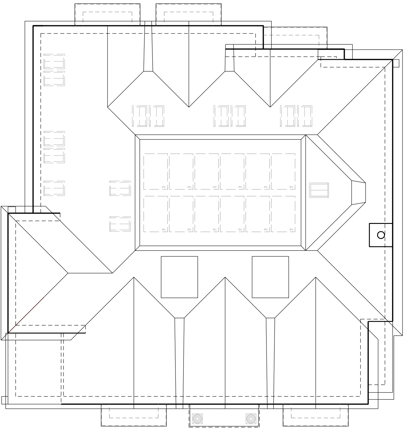
Roof Plan
