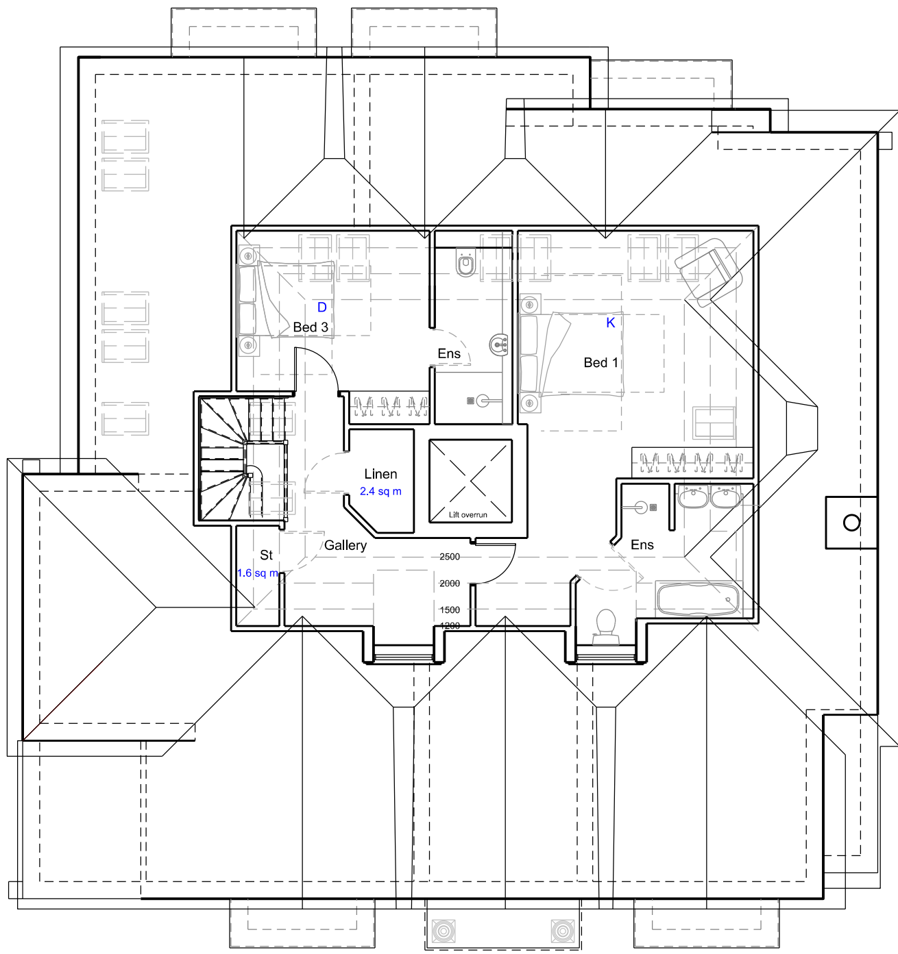
Second Floor
