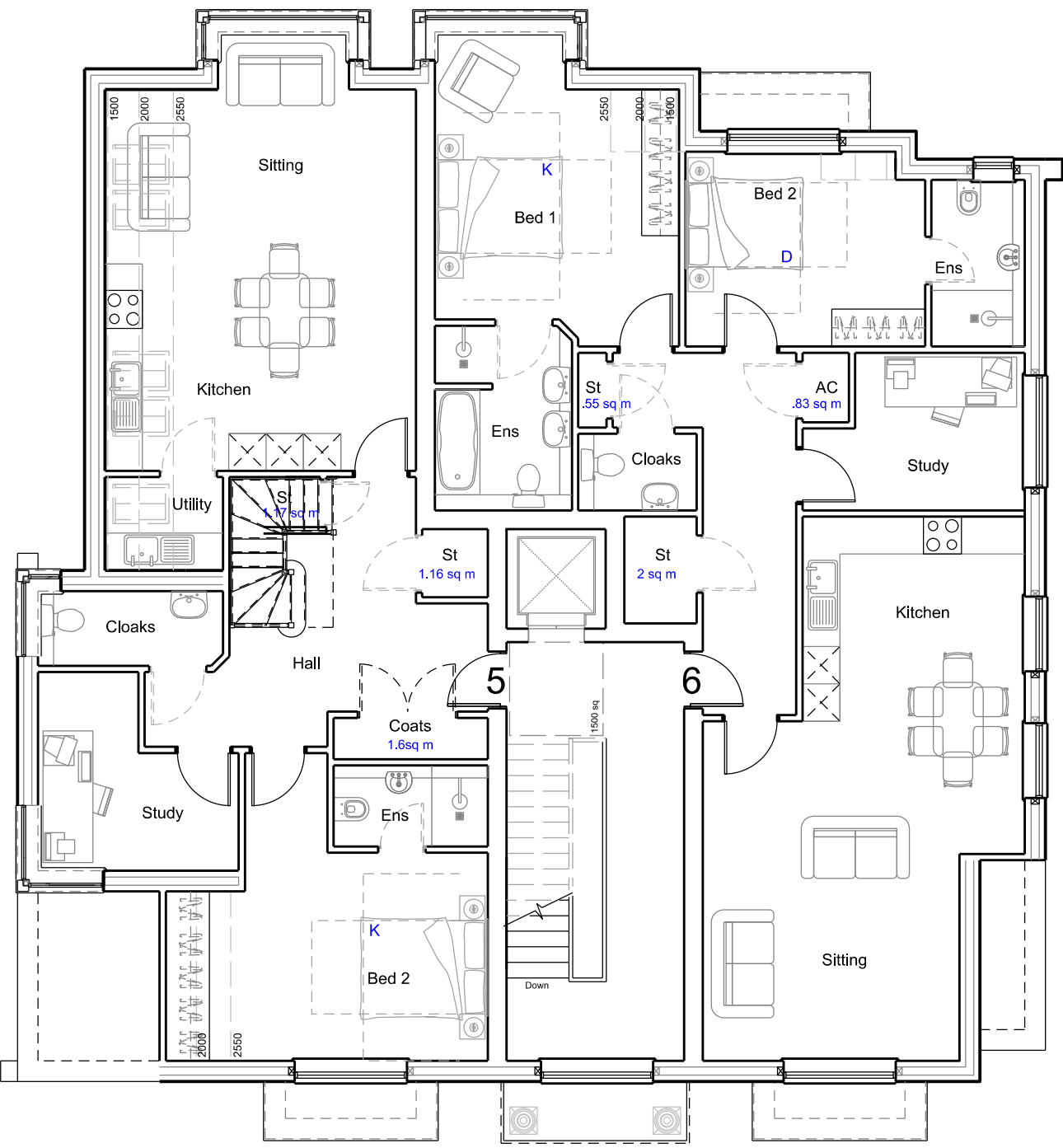
First Floor
