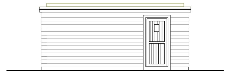
LHS ELEVATION
