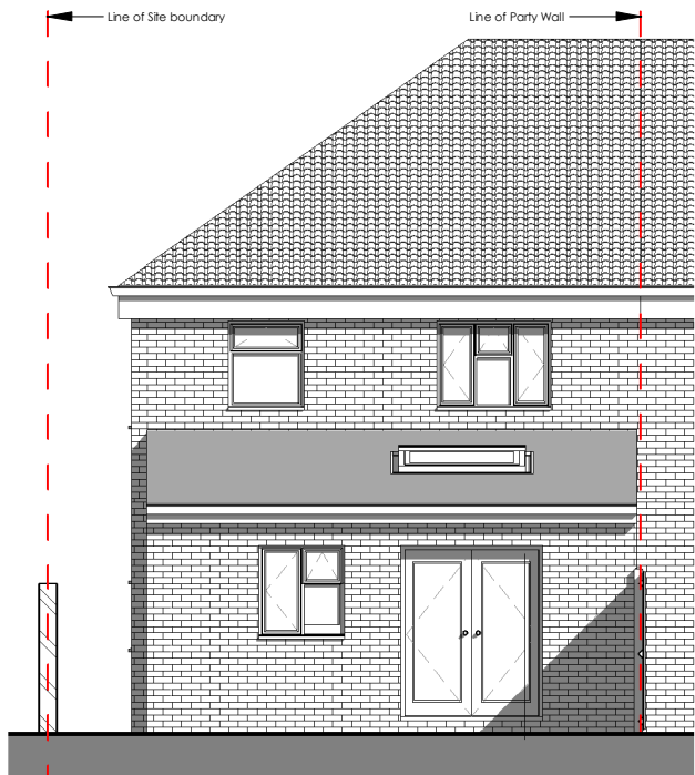
6 Existing Rear Elevation 2428-A-100 1 : 100
