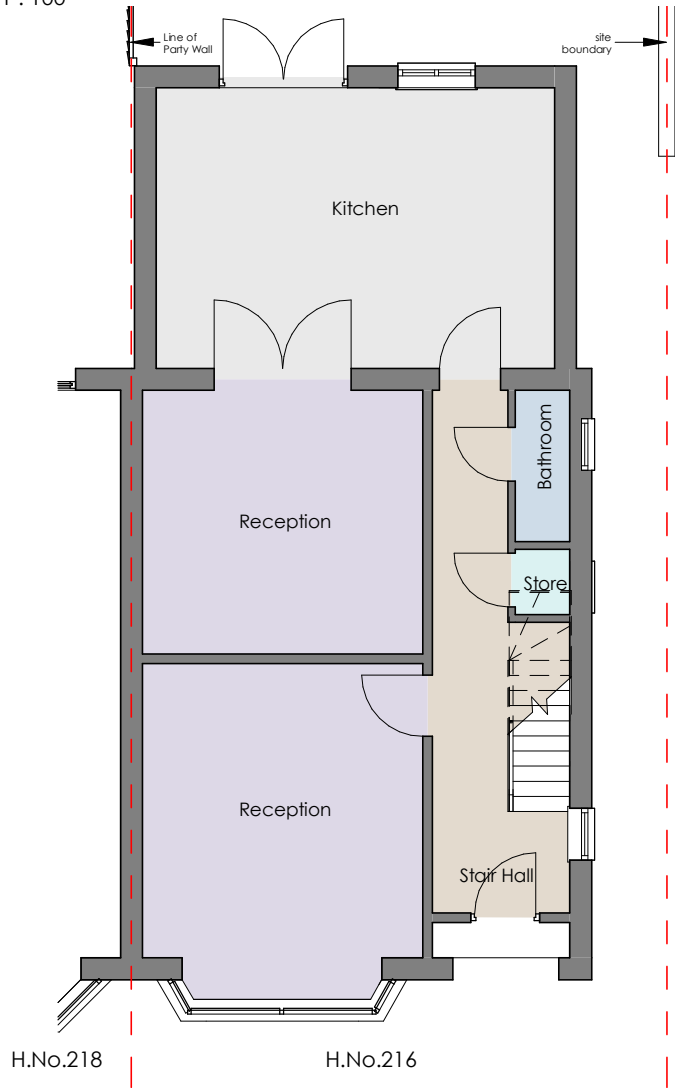
1 Existing Ground Floor 2428-A-100 1 : 100
