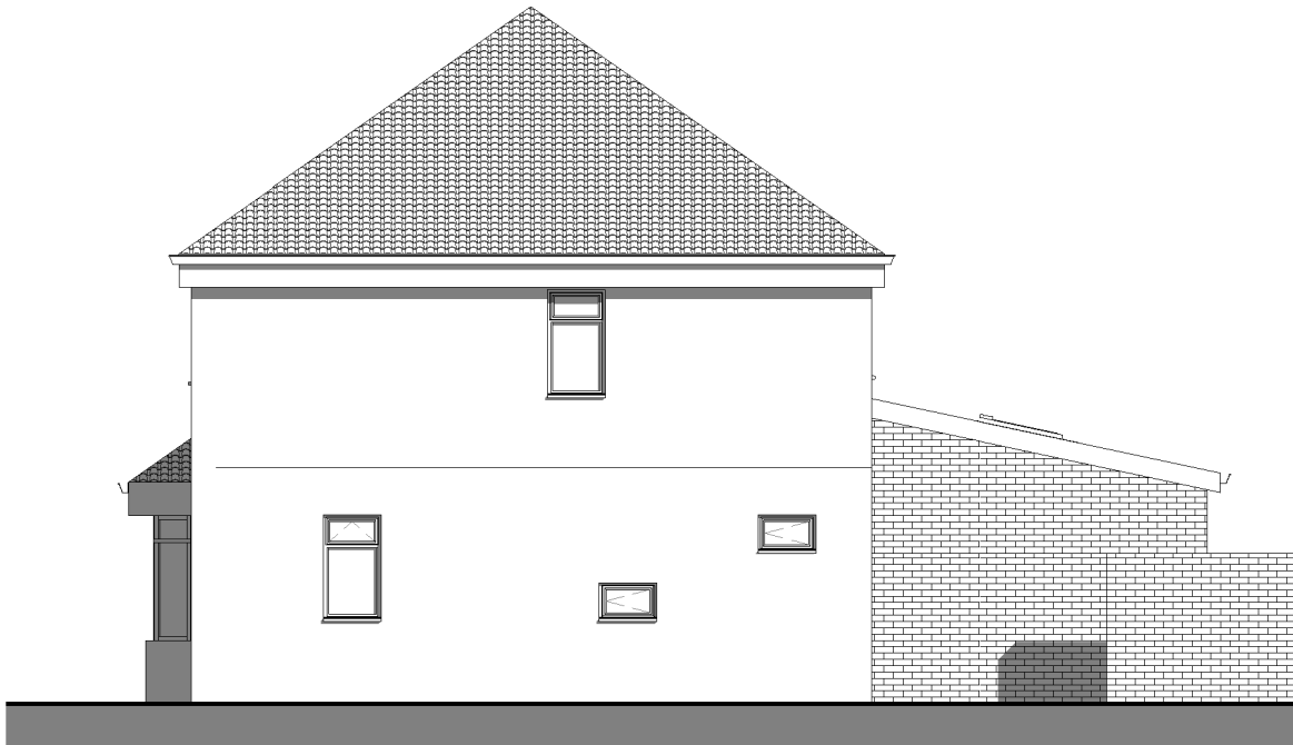
5 Existing Side Elevation 2428-A-100 1 : 100
