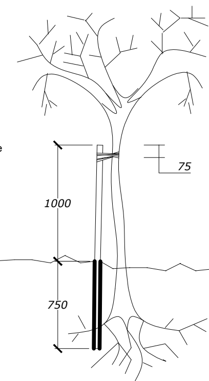
Staking for New Trees
