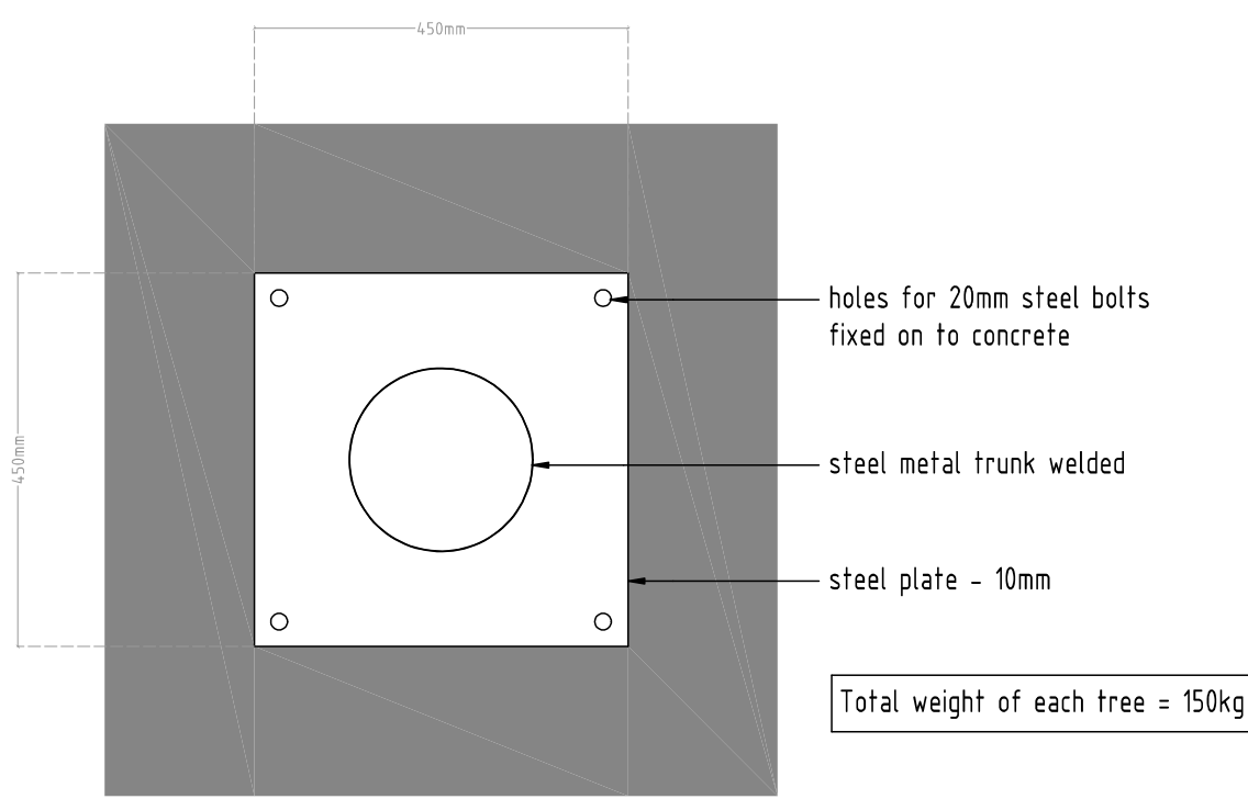
ARTIFICIAL TREE PLAN DETAIL SCALE 1:10
