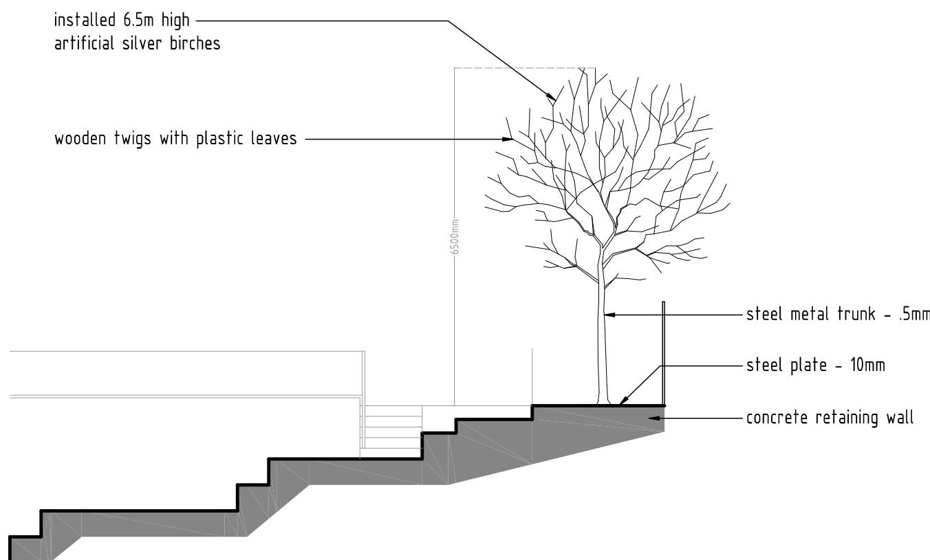
ARTIFICIAL TREES SECTION SCALE 1:100
