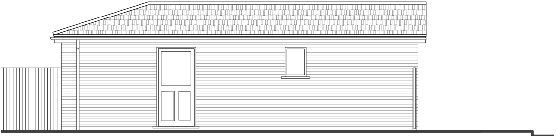
Side Elevation from No 43 , Proposed
