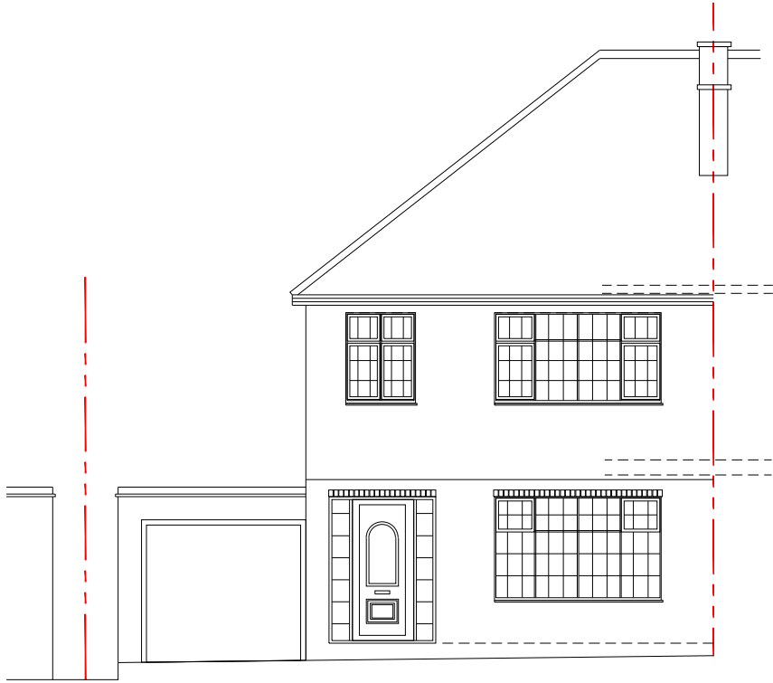
Front Elevation
