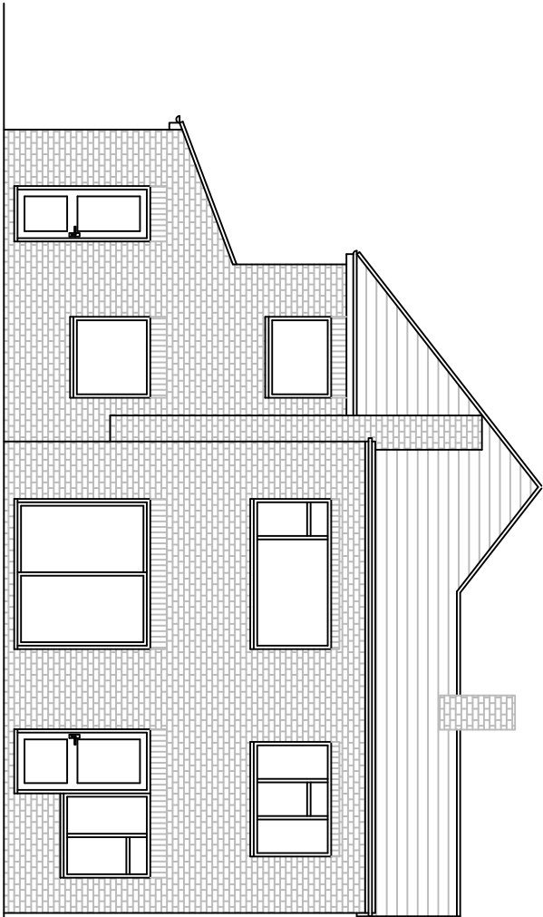
Rear (South) Elevation
