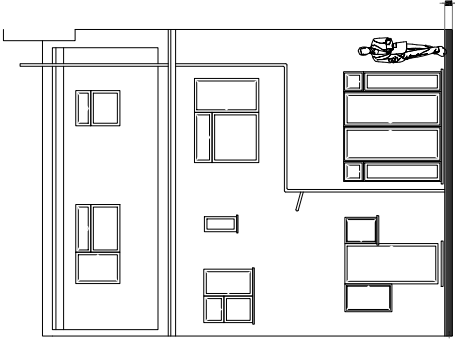
Rear Elevation Existing
