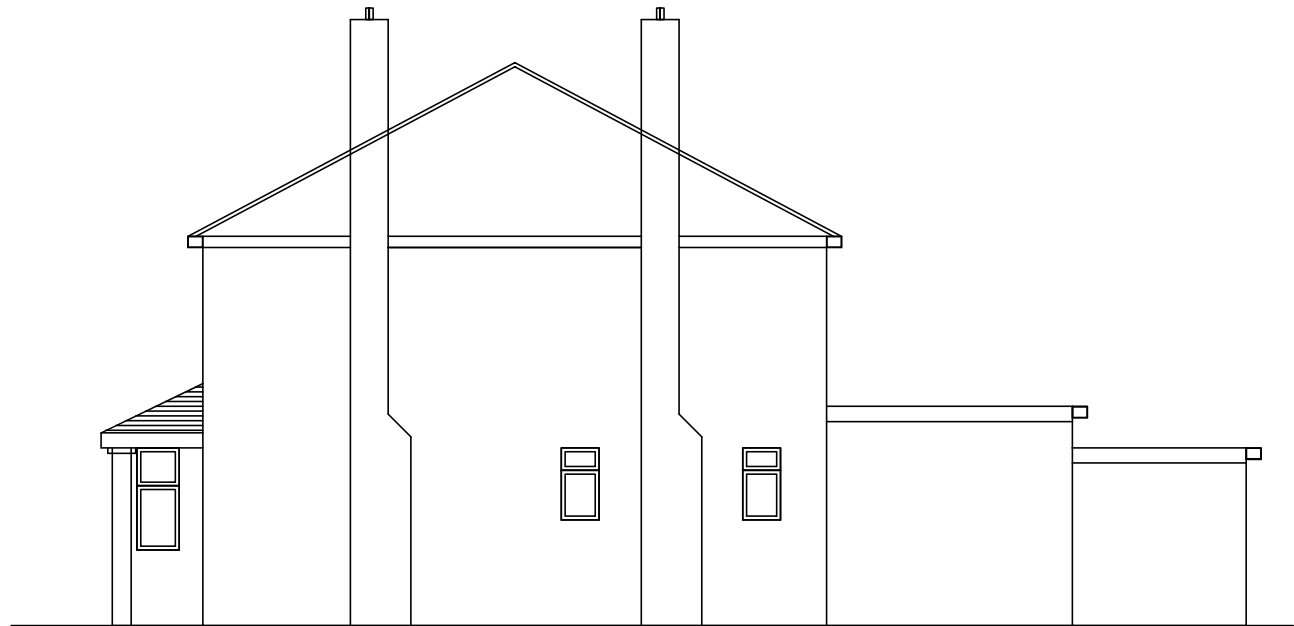
Existing Right Side Elevation
