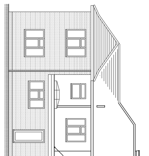
east elevation
