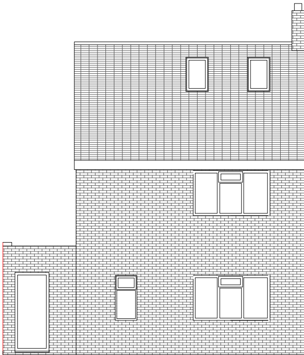
FRONT ELEVATION
