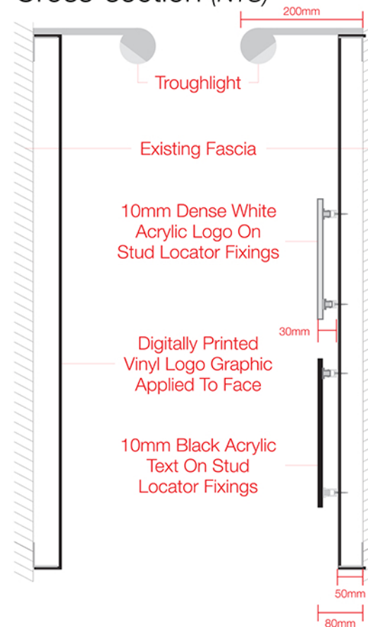
Cross-section (NTS)
