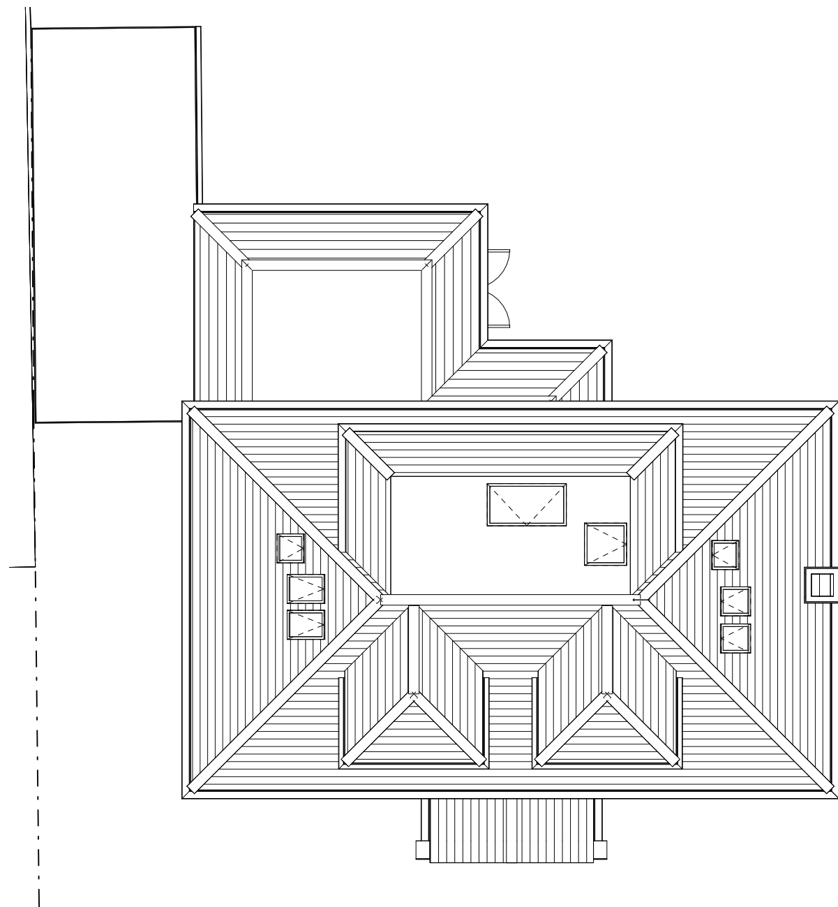
1 PROPOSED ROOF PLAN_
