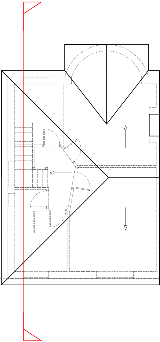
Roof plan existing
