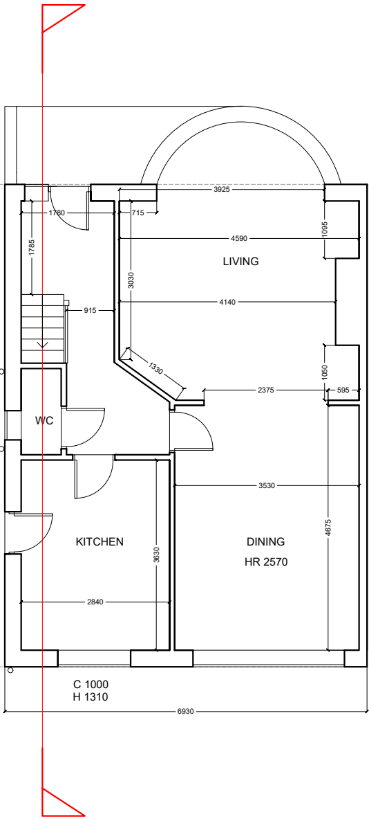
Ground floor existing
