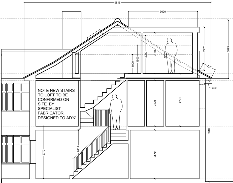
Long section proposed
