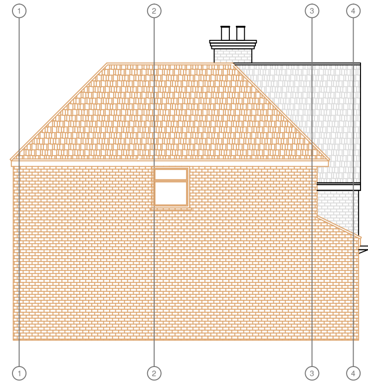
PROPOSED LEFT SIDE ELEVATION
