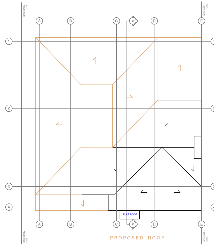
PROPOSED ROOF
