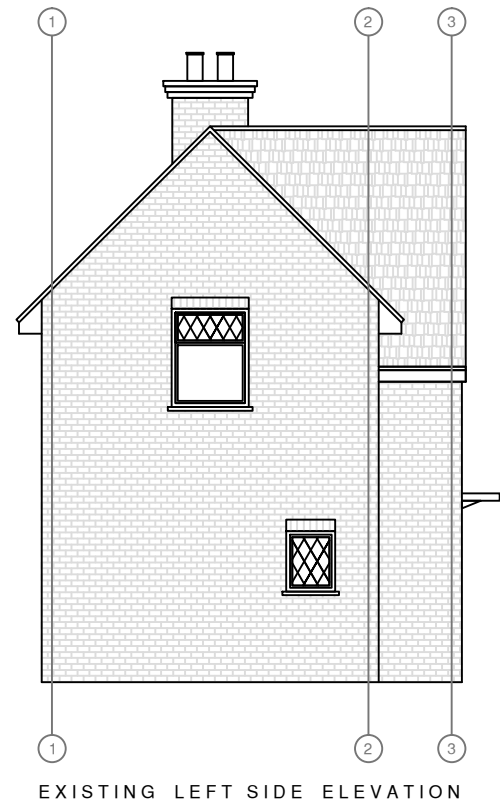
EXISTING LEFT SIDE ELEVATION
