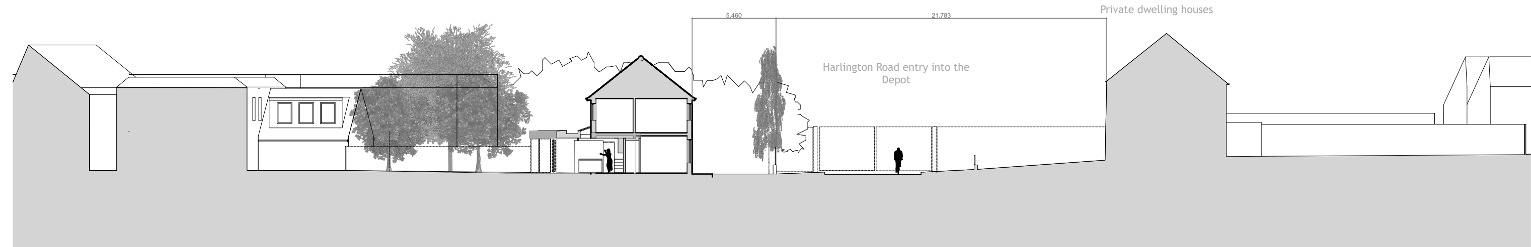
2.Proposed Site Section
