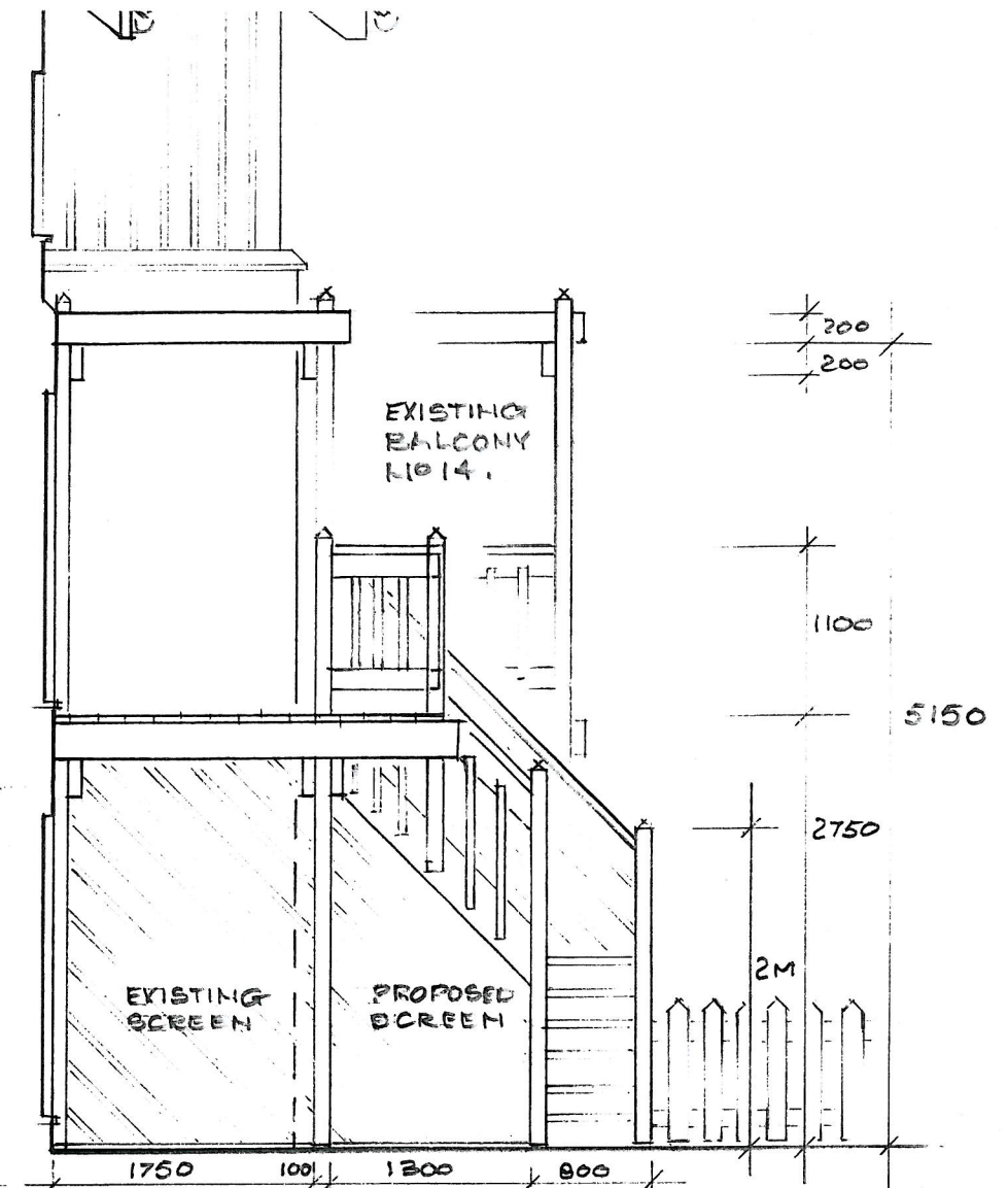
SECTION THRO EXTENDED BALCONY AND NEW STAIRCASE AND PROPOSED NEWSIDE SCREEN
