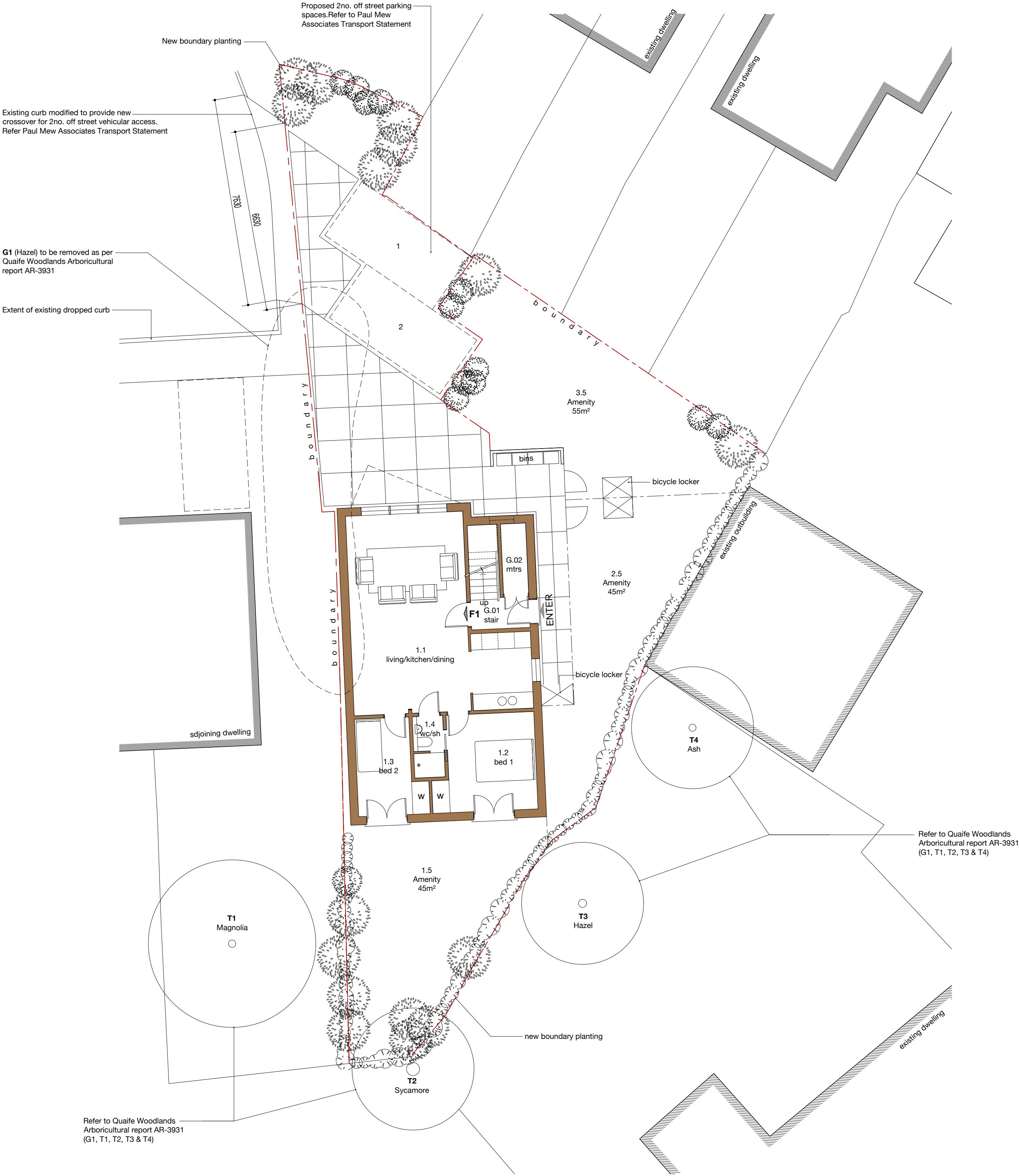
PROPOSED GROUND 1:100 GIFA 63m²
