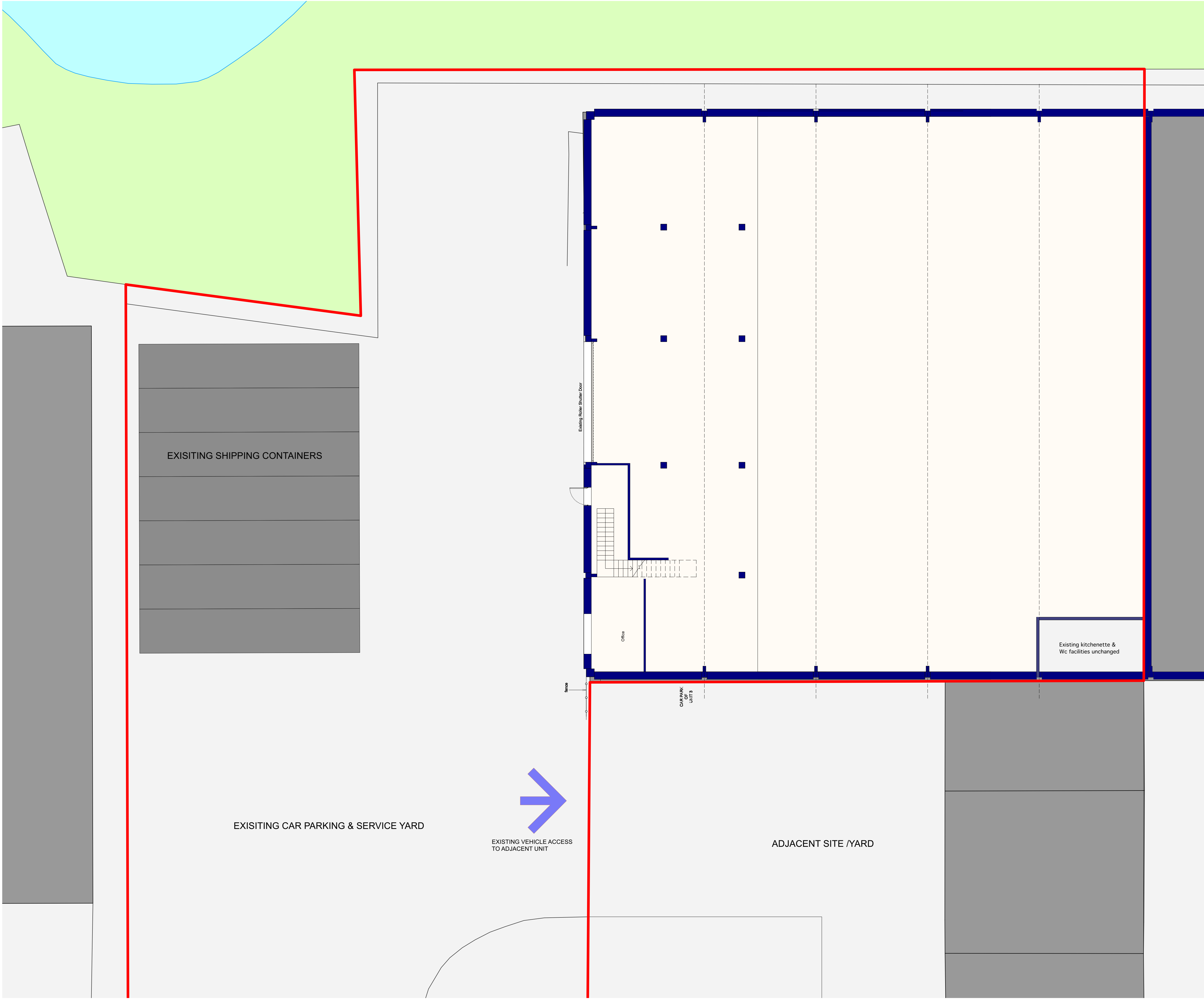
1 EXISTING GROUND FLOOR PLAN Scale: 1:100
