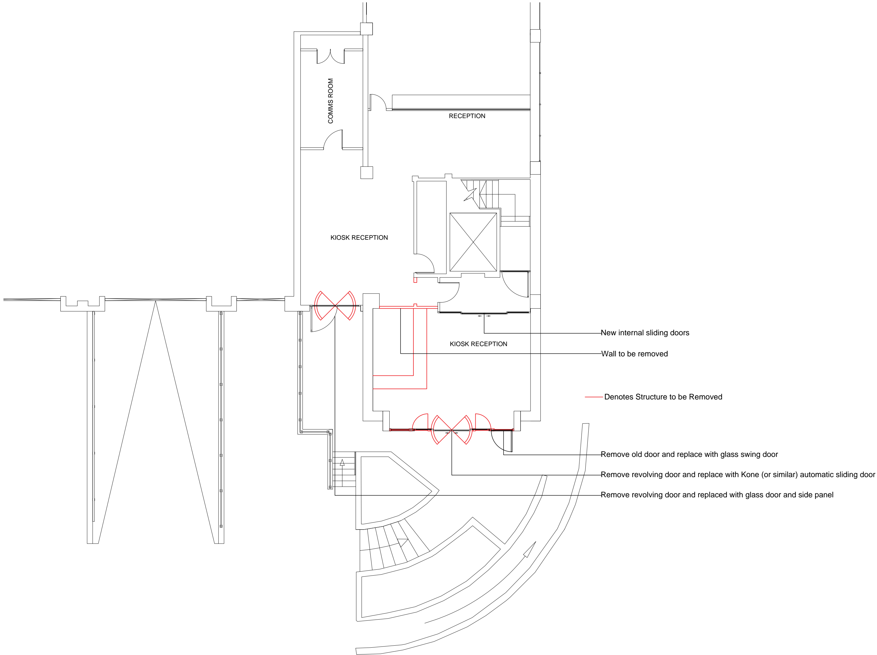
Proposed Reception Plan Scale 1:100 at A1
