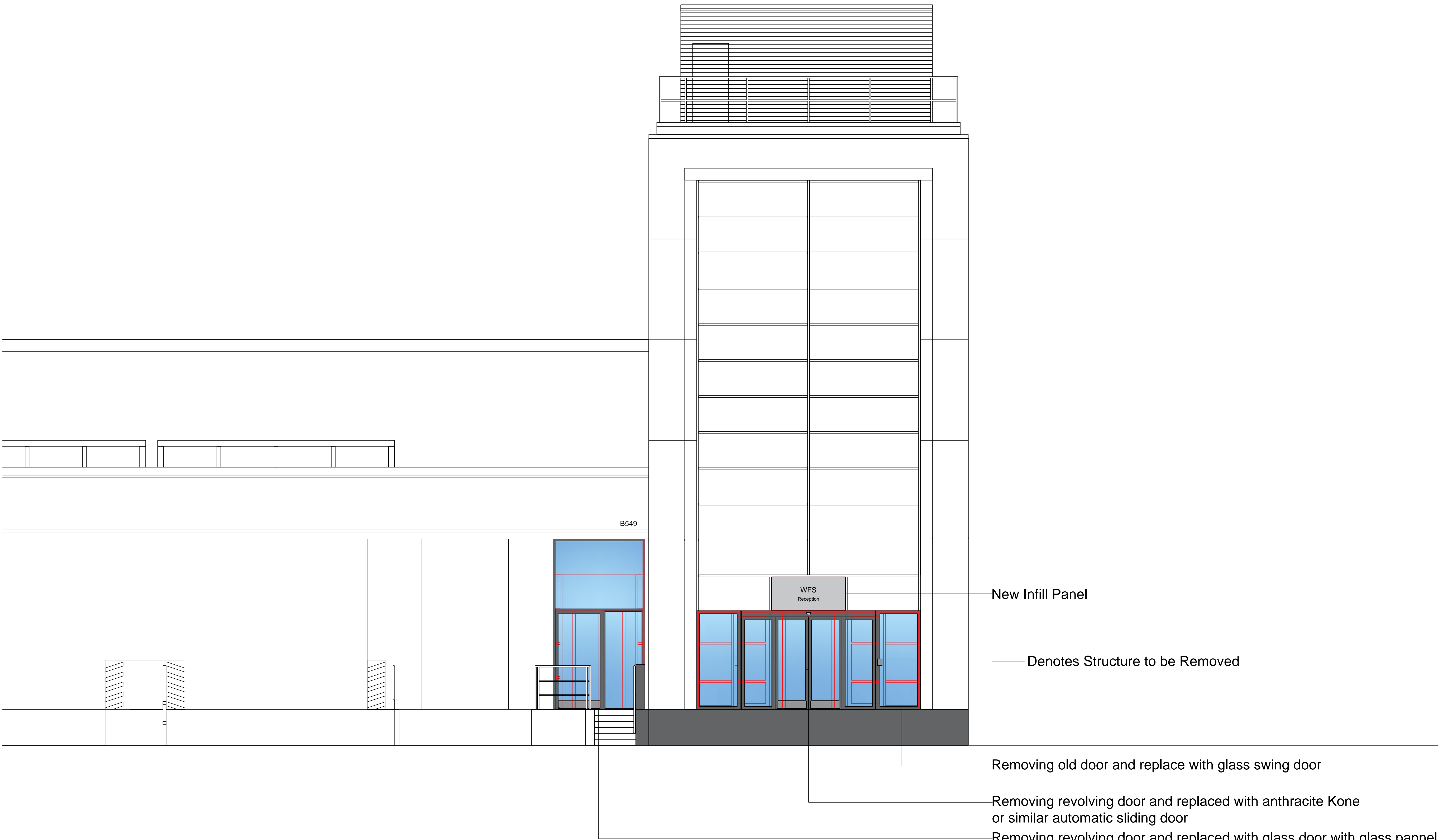
Proposed Front West Elevation Scale 1:50 at A1
