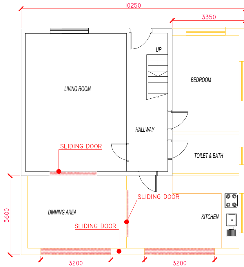
Proposed Ground Floor Layout
