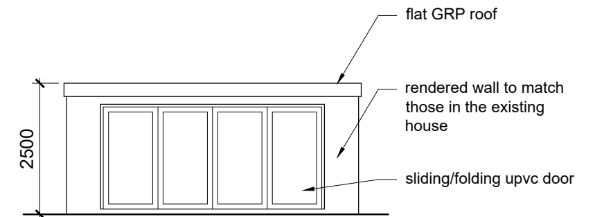
PROPOSED ELEVATION F
