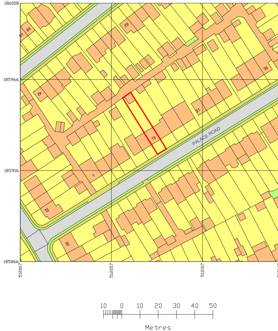
LOCATION PLAN 1:1250
