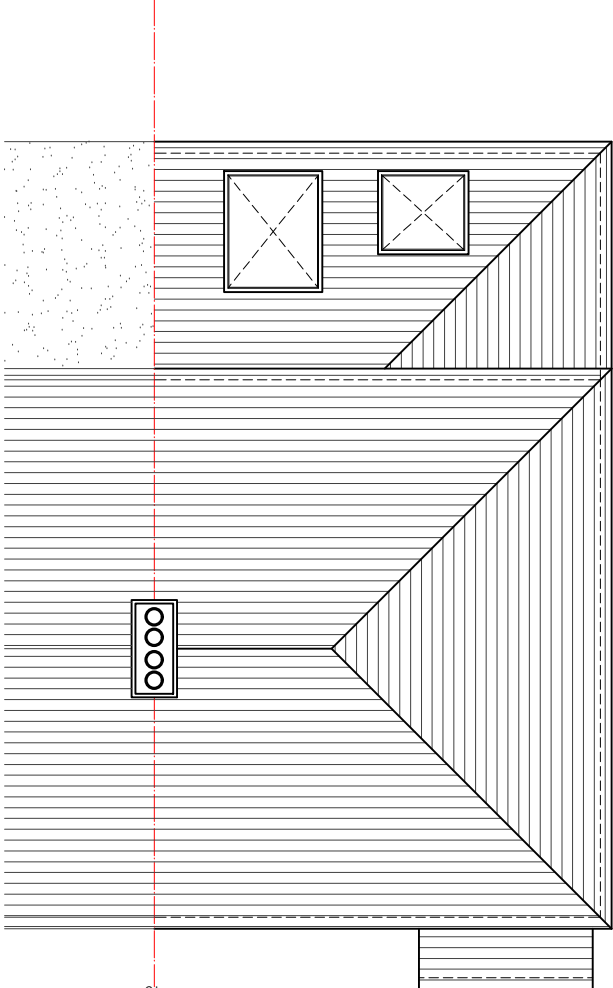
02 - ROOF PLAN
