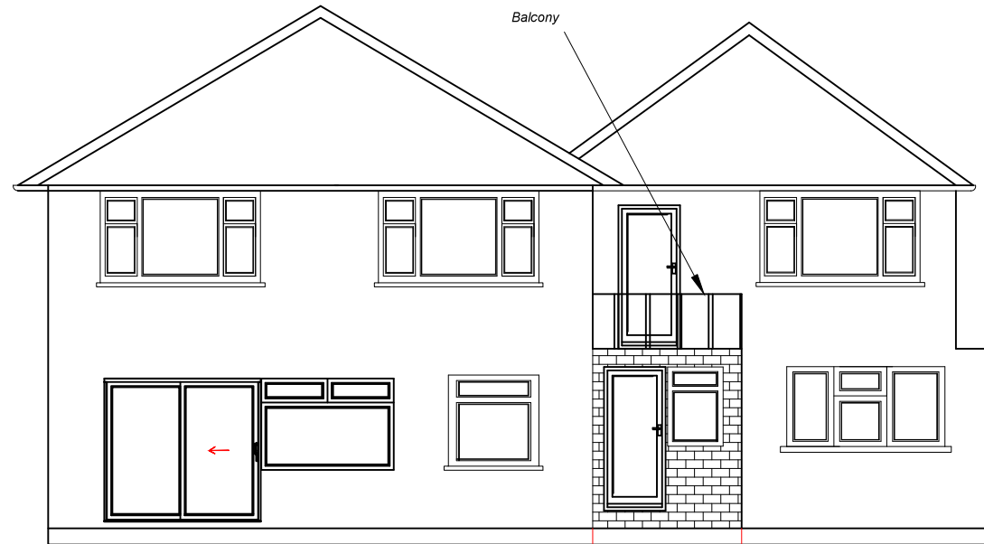
Proposed back elevation
